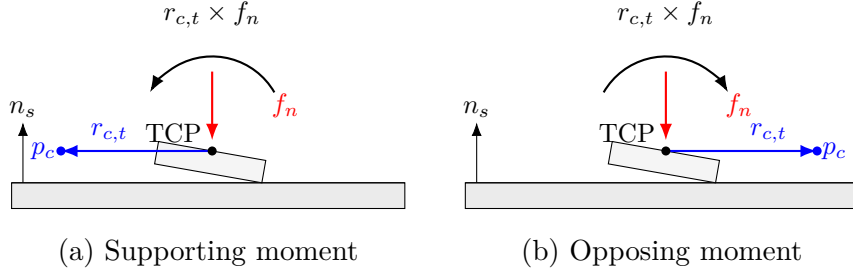
Figure 2.3: Normal-force contribution for (a) the selected tangential displacement and (b) its reversal.
