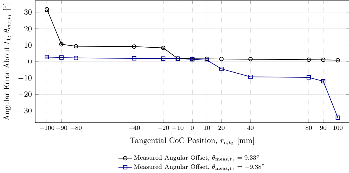
Figure 5.7: Angular error by tangential CoC position.
