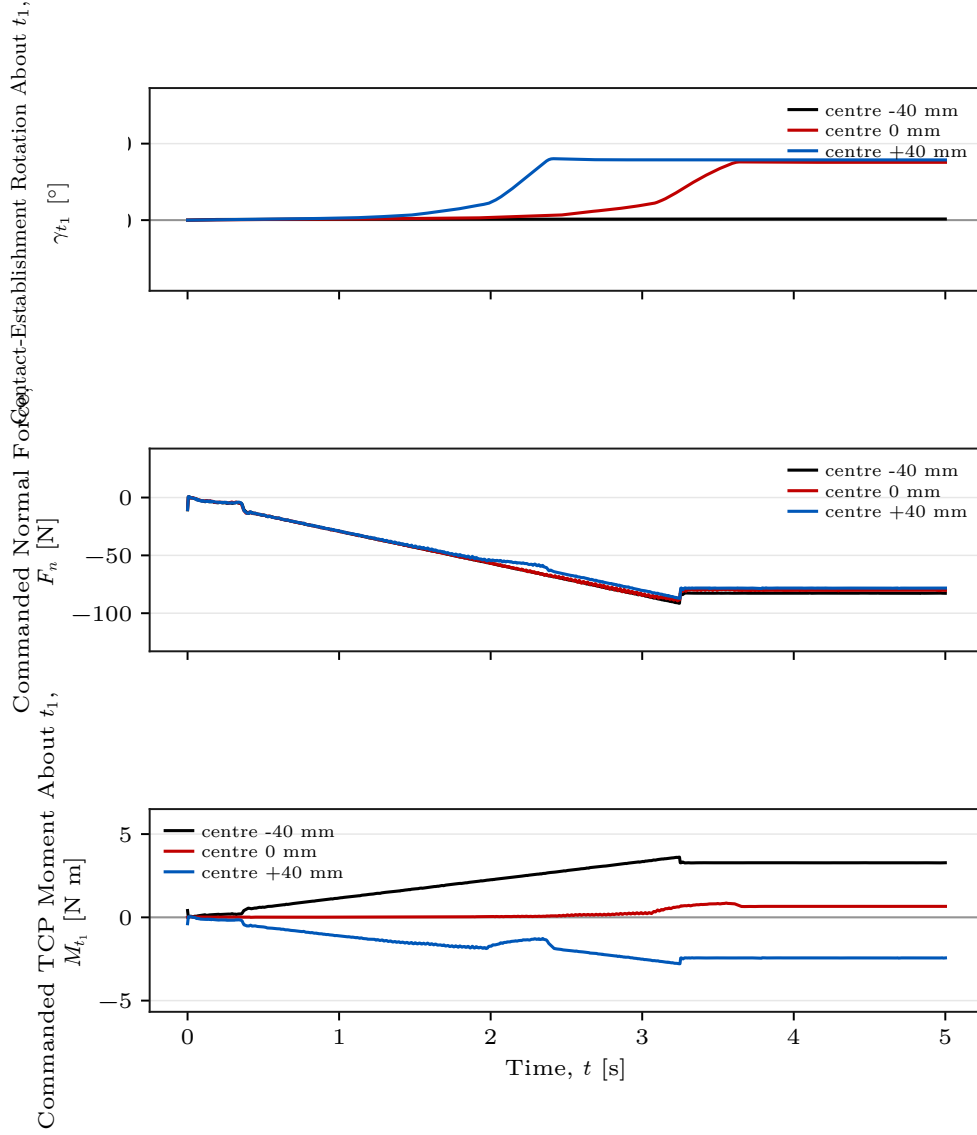
Figure 5.5: Measured contact-establishment rotation, commanded normal force, and commanded TCP moment for three tangential CoC positions.
