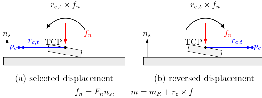
Figure 2.4: Normal-force contribution to the compliance-centre coupling moment for opposite tangential displacements: (a) the displacement selected from the orientation offset; (b) the displacement with the opposite sign.
