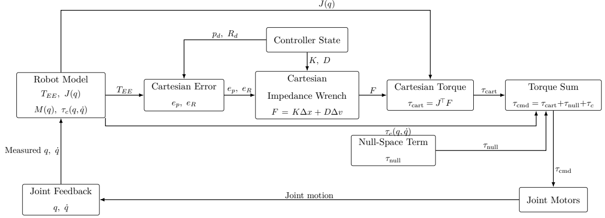
Figure 3.2: Torque contributions combined in one control cycle.
