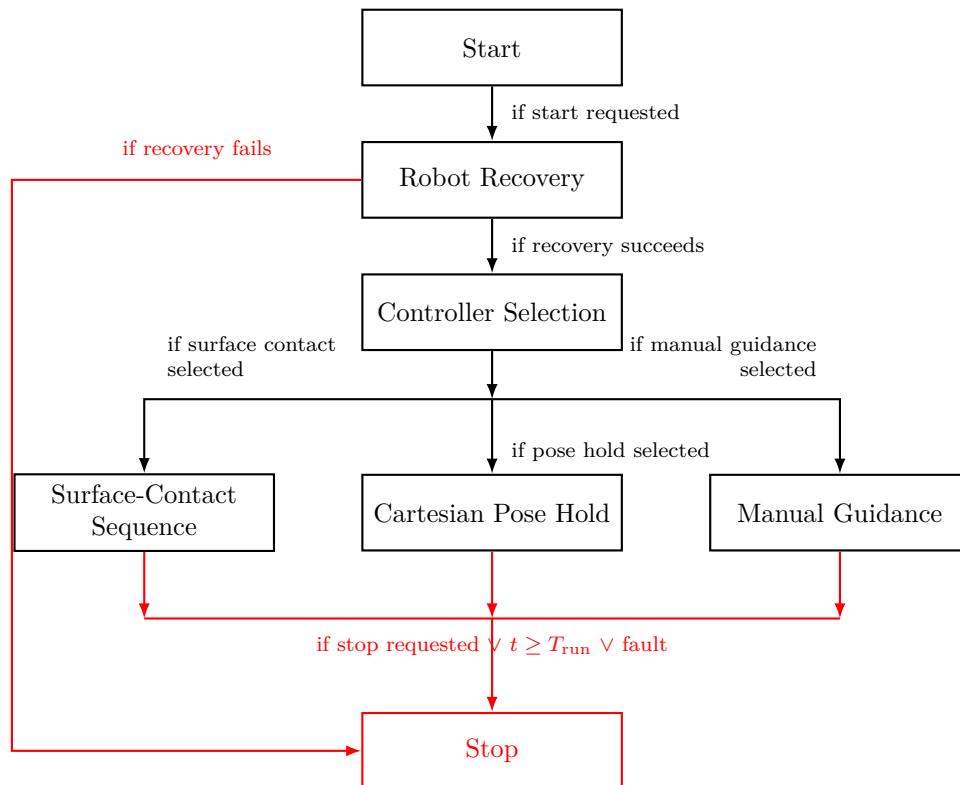
Figure 3.1: Controller operating-state flow.
