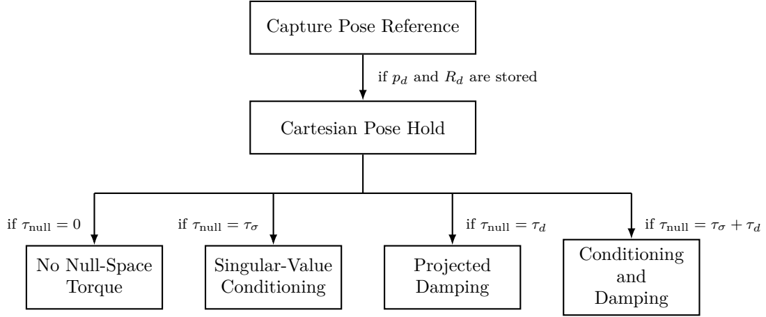
Figure 3.7: Cartesian pose hold with four selectable null-space configurations.
