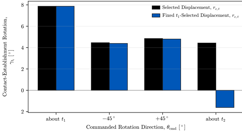
Figure D.4: Contact-establishment rotation with the direction-selected and fixed displacements.
