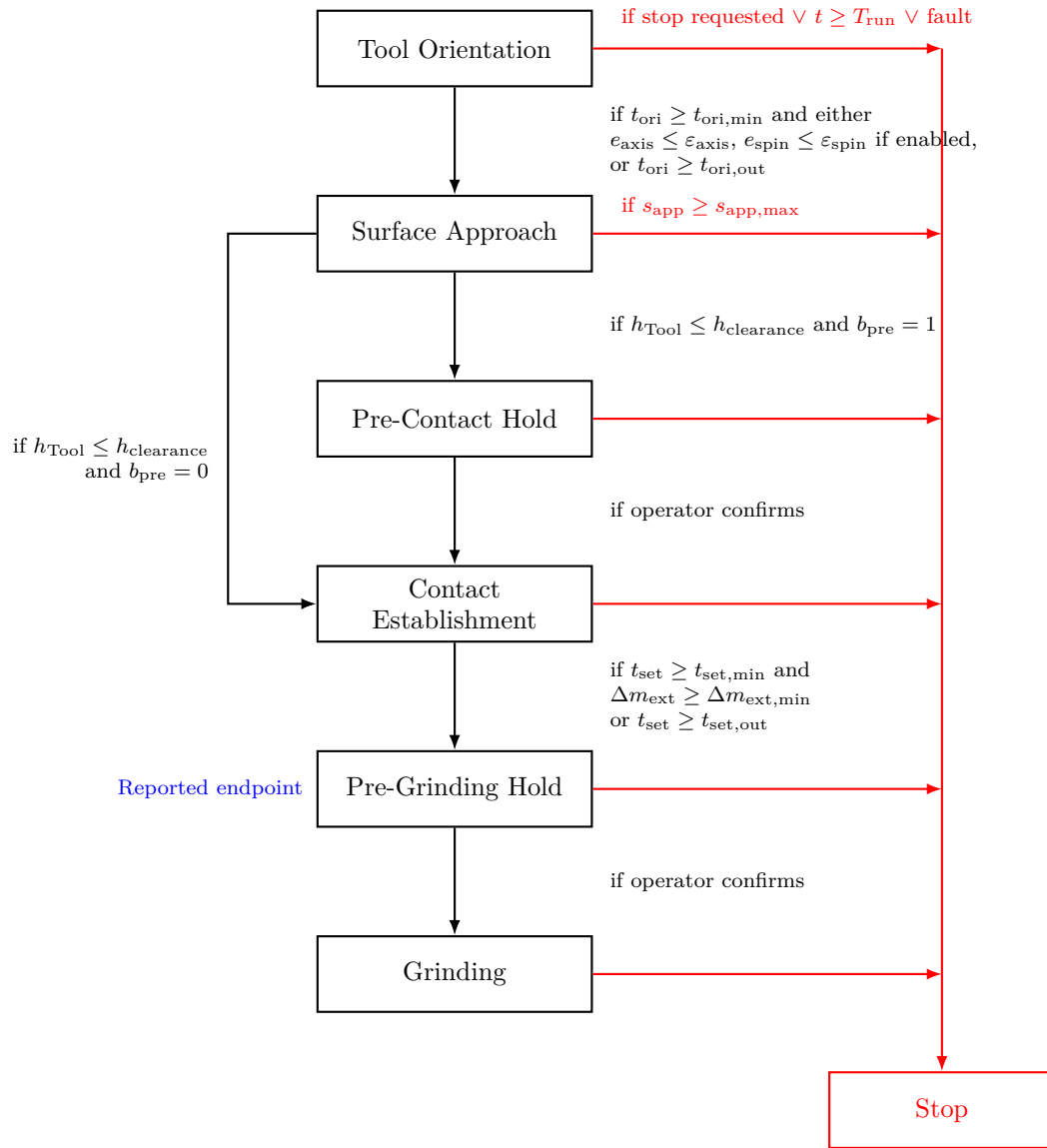
Figure 3.3: Surface-contact state transitions.
