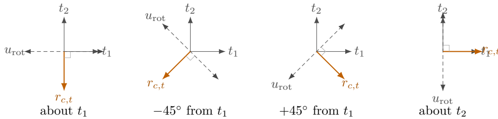
Figure 4.4: Selected tangential lever for each commanded rotation direction.
