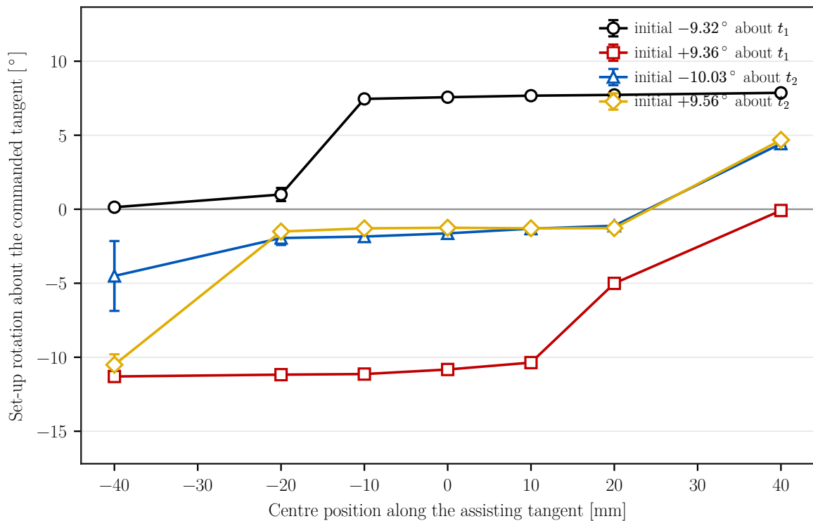
Figure 5.3: Signed set-up rotation about the commanded tangent by centre position, for both surface tangents and both signs of the commanded offset.
