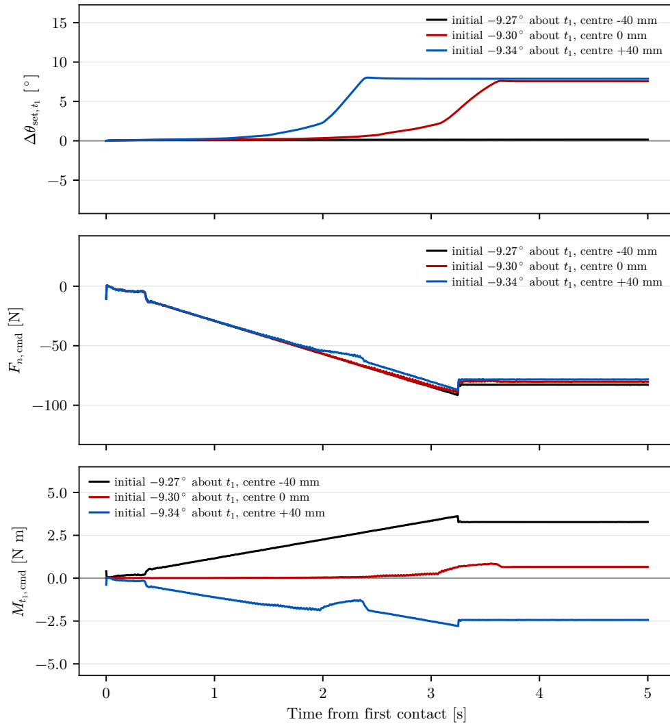
Figure 5.4: Set-up rotation \Delta\theta_{\text{set},t_1} , commanded normal force F_{n,\text{cmd}} , and commanded TCP moment M_{t_1,\text{cmd}} for three centre positions. All conditions carry a commanded offset of +10^\circ about t_1 . The legends state the measured orientation at first contact.
