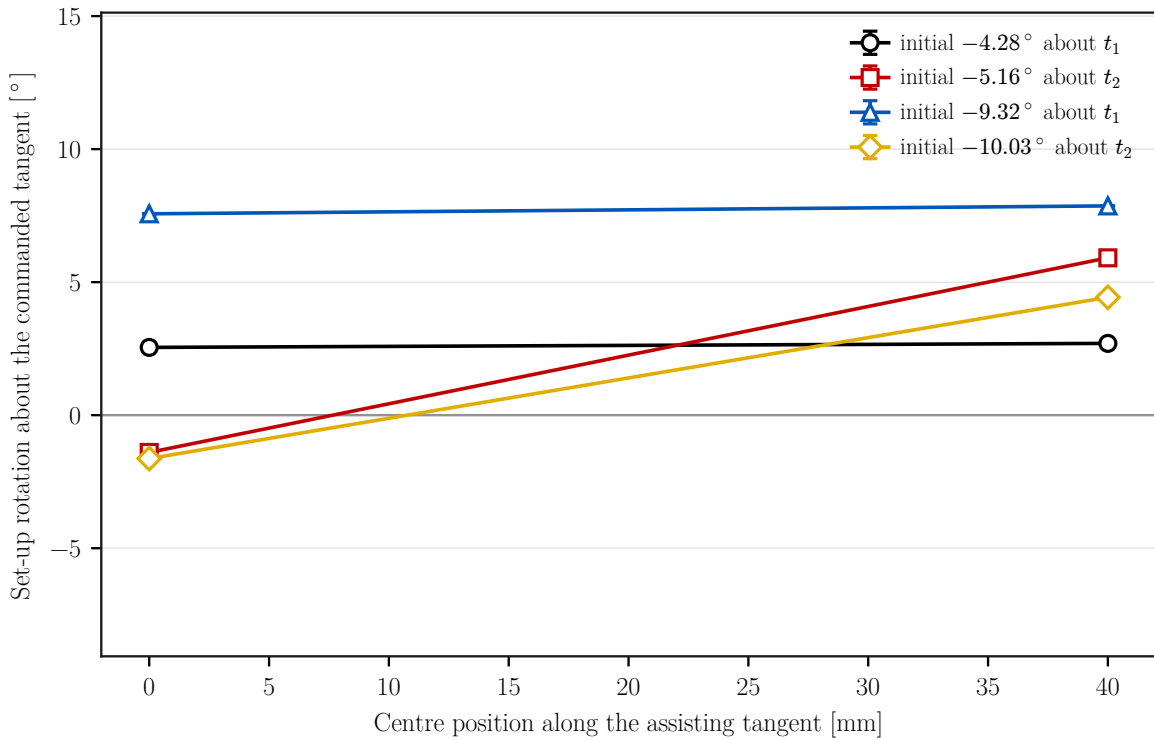
Figure 5.7: Signed set-up rotation about the commanded tangent at both commanded magnitudes, by centre position along the assisting tangent.
