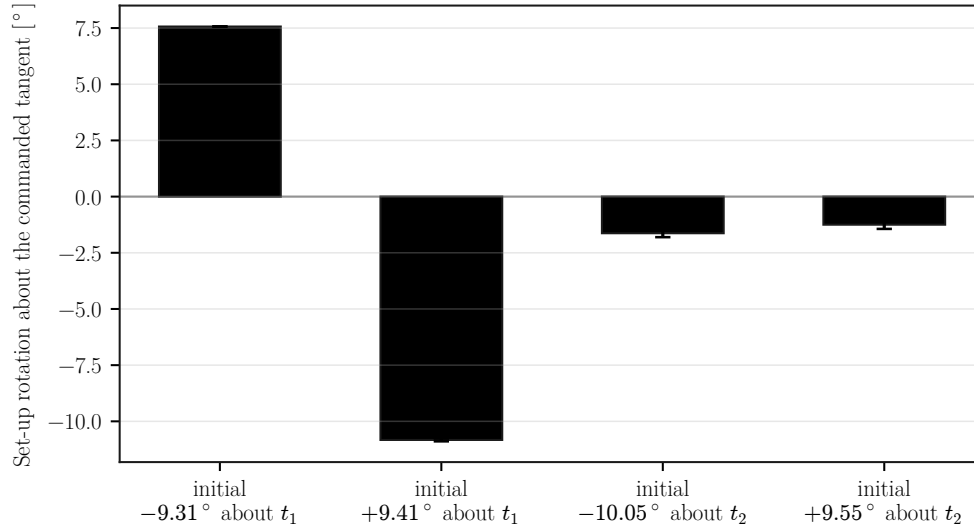
Figure 5.2: Signed set-up rotation about the commanded tangent with the centre of compliance on the TCP.
