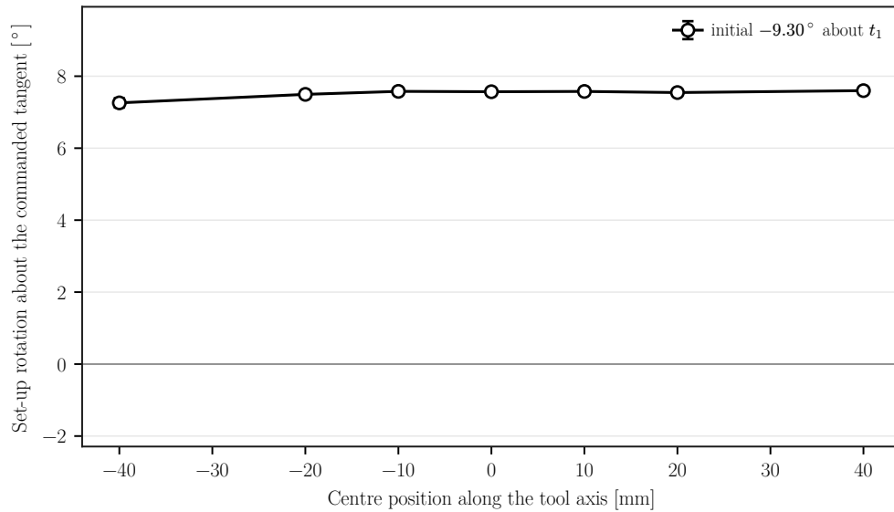
Figure 5.6: Signed set-up rotation about t_1 by centre position along the tool axis.
