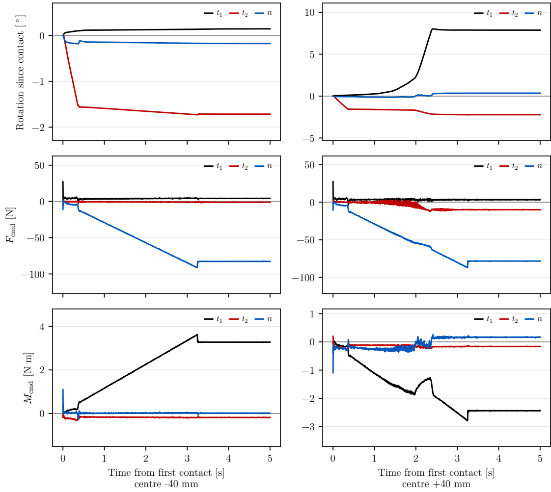
Figure 5.5: Surface-frame components of the set-up rotation, commanded Cartesian force, and commanded TCP moment for the two outer Case-E positions.
