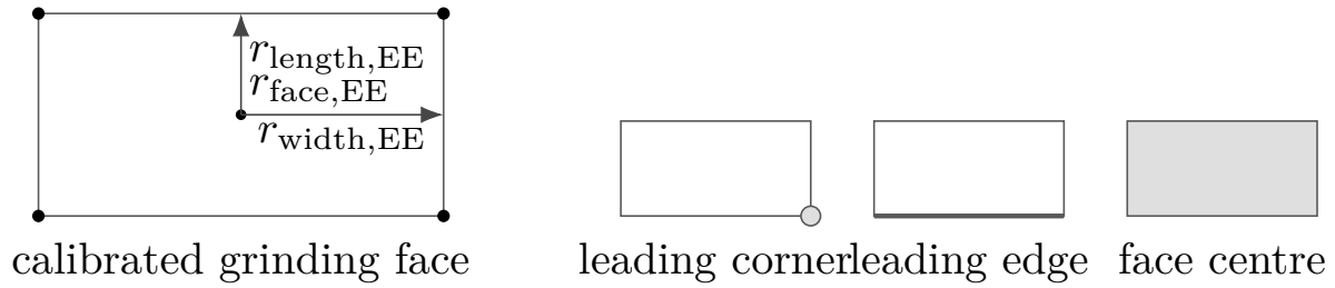
Figure 3.2: Grinding-face geometry and the selected leading feature.
