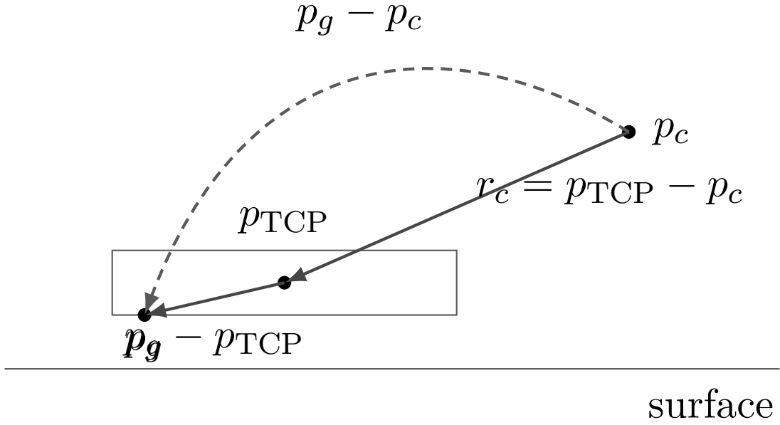
Figure 3.3: Selected face point, tool centre point, and centre of compliance.
