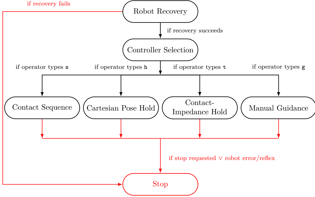
Figure 3.1: Principal controller operating-state flow.
