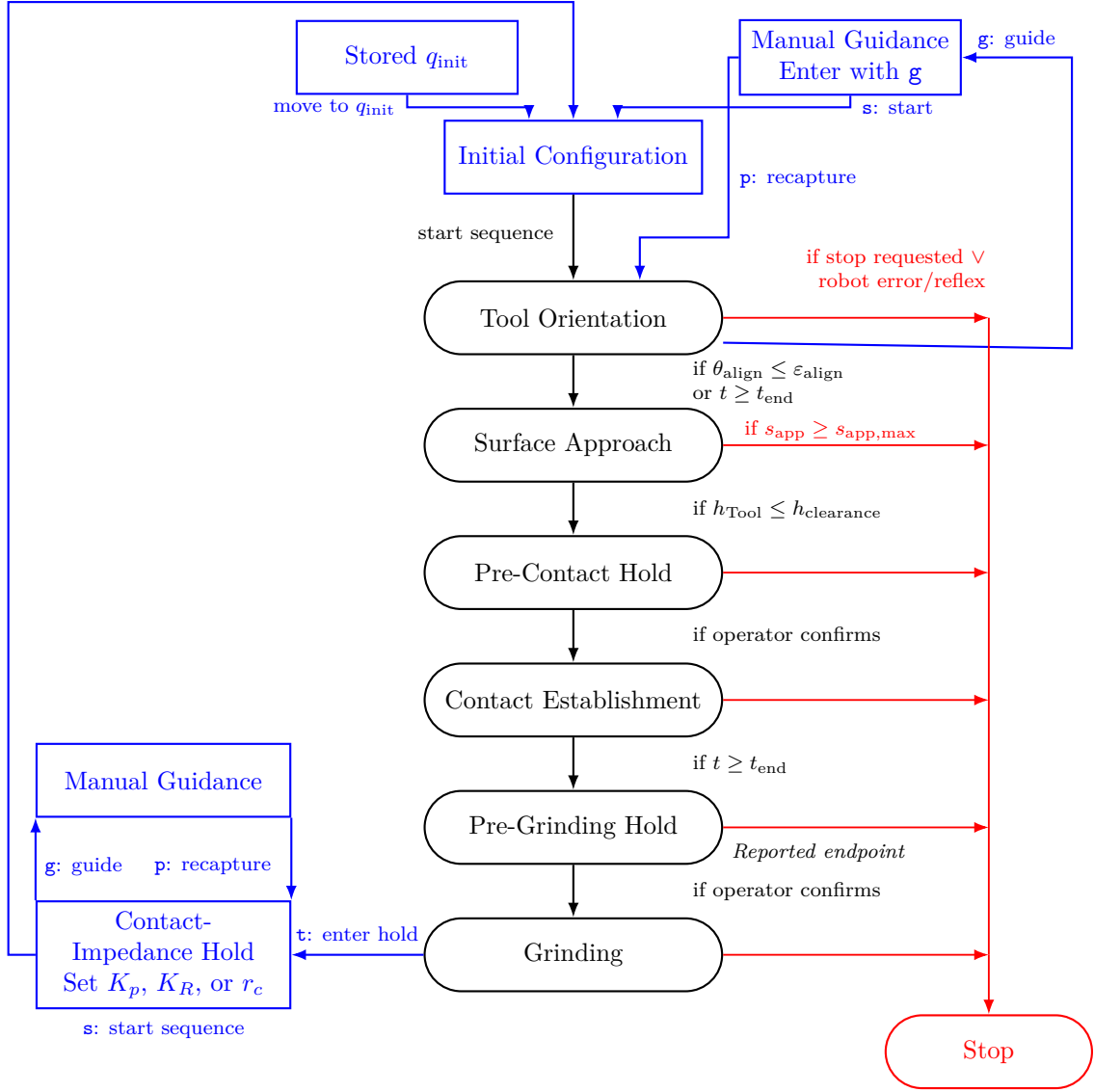
Figure 3.3: Surface-contact sequence and contact-impedance tuning loop.
