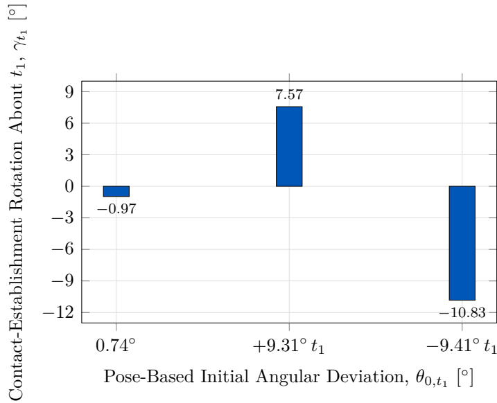
Figure 5.1: Measured contact-establishment rotation with the CoC at the TCP.
