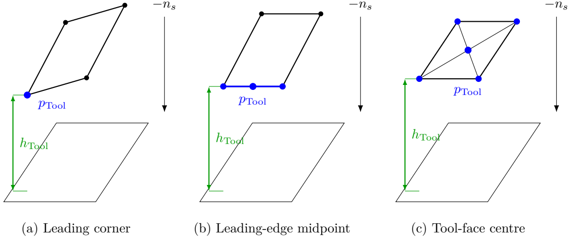
Figure 3.5: Principal selected tool points for the rectangular tool face.
