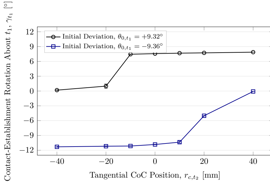
Figure 5.4: Contact-establishment rotation by tangential CoC position (mean \pm SD).
