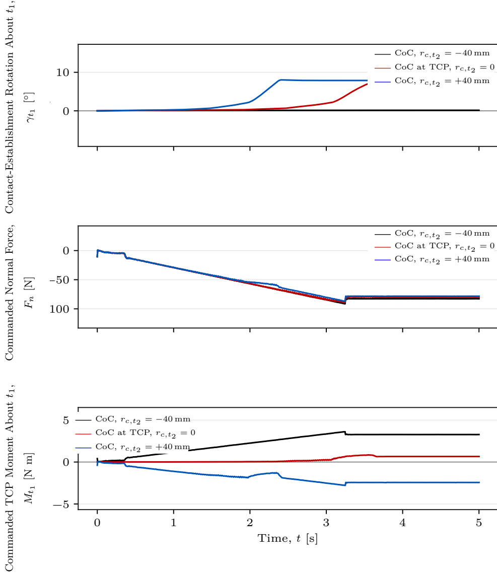
Figure 5.5: Contact response and commanded wrench by CoC position.
