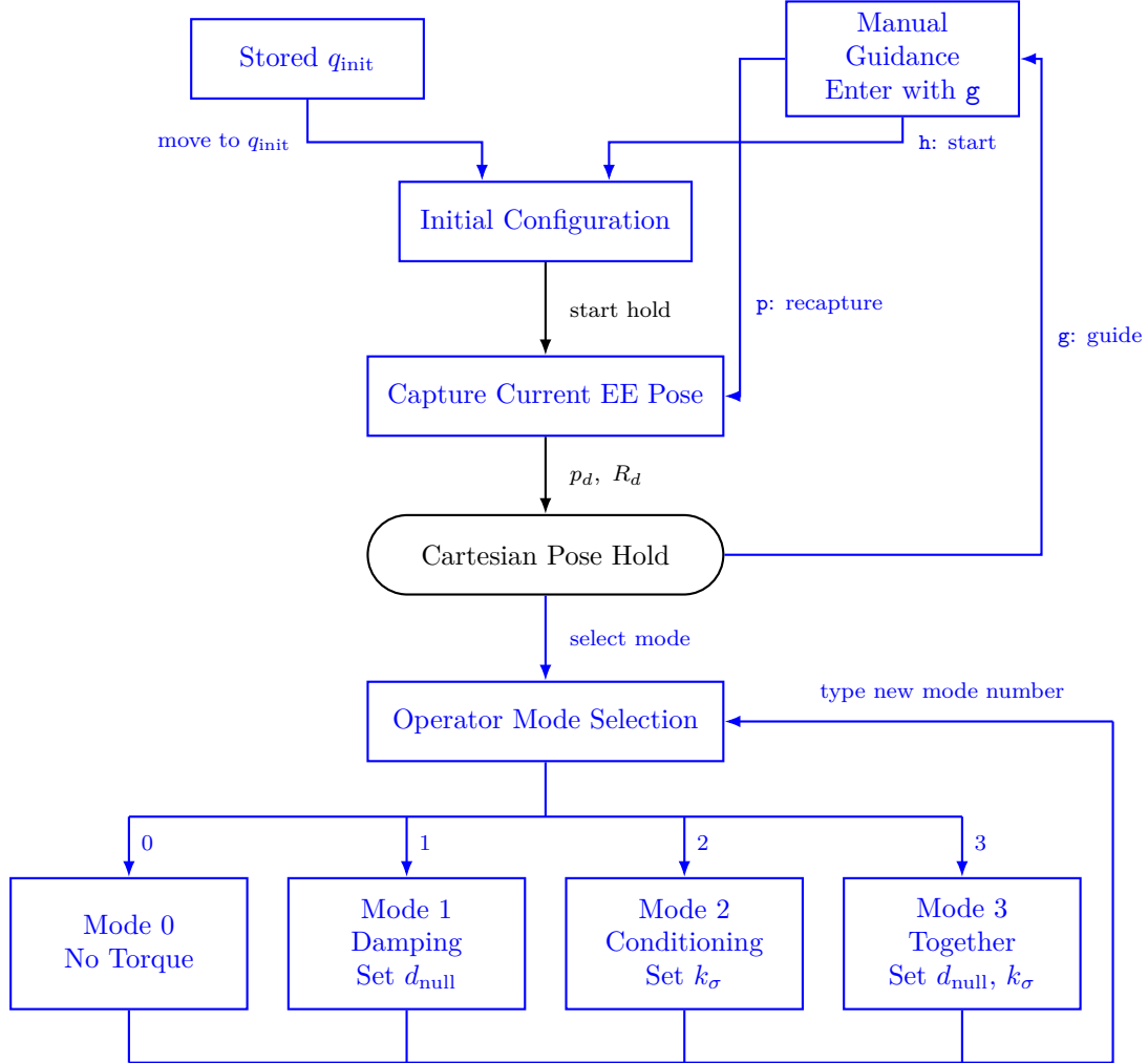
Figure 3.7: Operator-selectable null-space modes in Cartesian pose hold.
