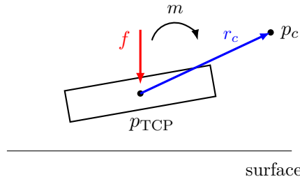
Figure 2.2: Compliance-centre displacement and commanded TCP moment.
