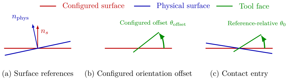
Figure 1.1: Surface reference, orientation offset, and contact entry. +
