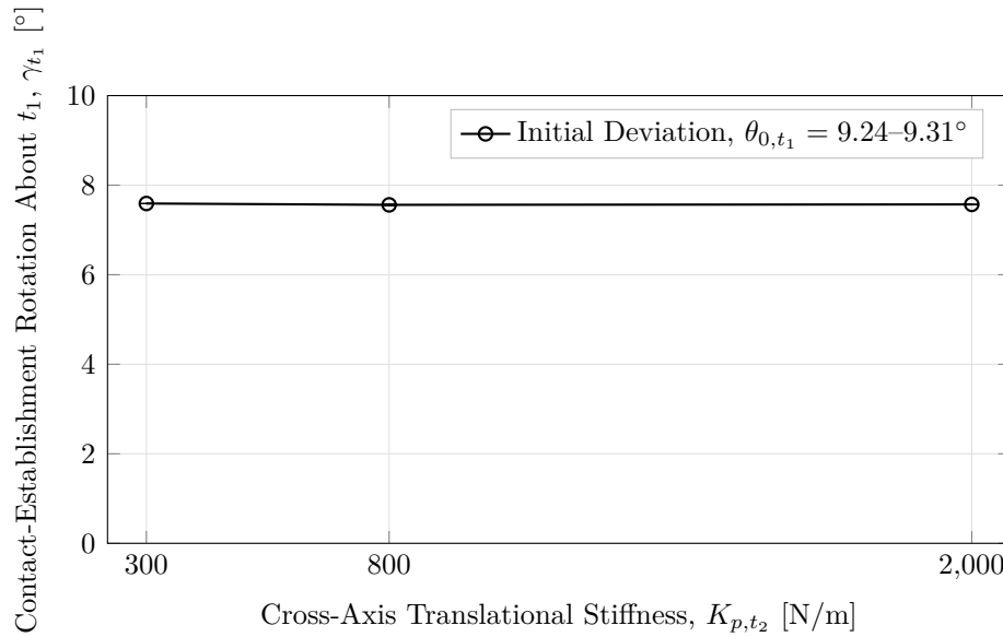
Figure 5.3: Measured contact-establishment rotation by cross-axis translational stiffness.
