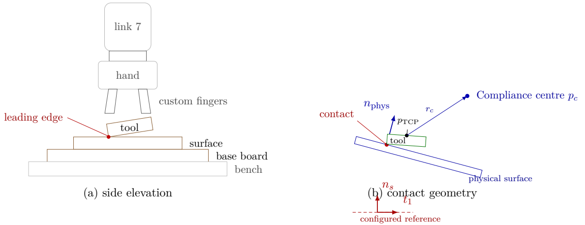
Figure 4.1: Experimental system and surface-frame contact geometry.
