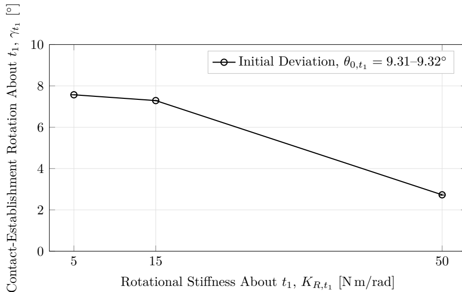
Figure 5.2: Measured contact-establishment rotation by rotational stiffness.
