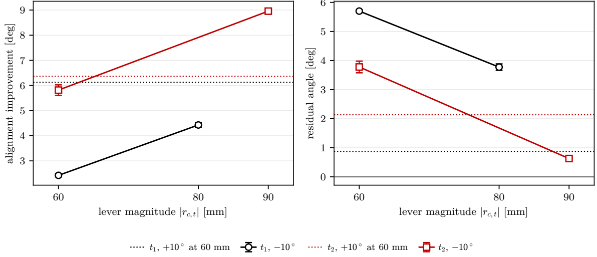
Figure 5.7: Reversed-tilt response at the extended lever magnitudes.
