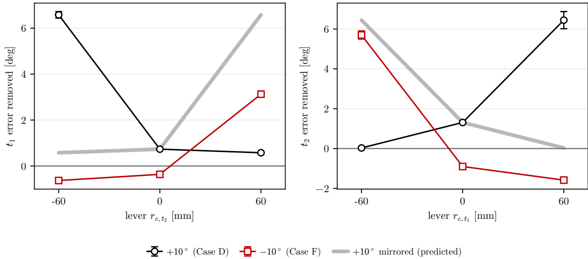
Figure 5.6: Alignment improvement at both tilt signs, by compliance-centre lever.
