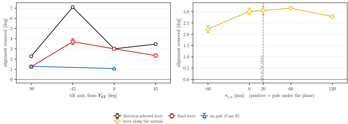
Figure 5.9: Alignment response by tilt direction and by normal lever coordinate.
