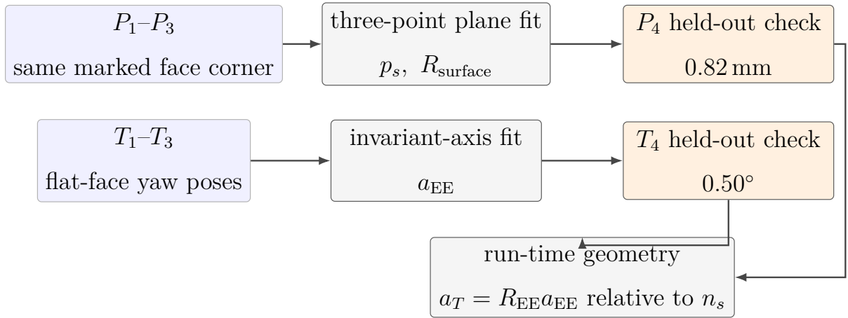
Figure 4.2: Independent calibration and validation flow.
