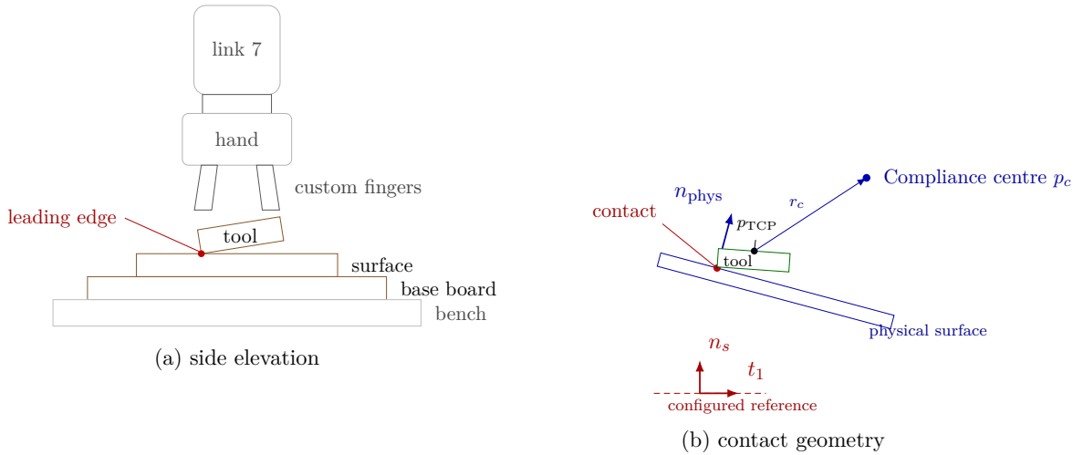
Figure 4.1: Experimental system and surface-frame contact geometry.
