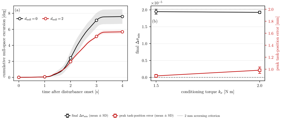
Figure 5.6: Automatic null-space response under the point-force equivalent.
