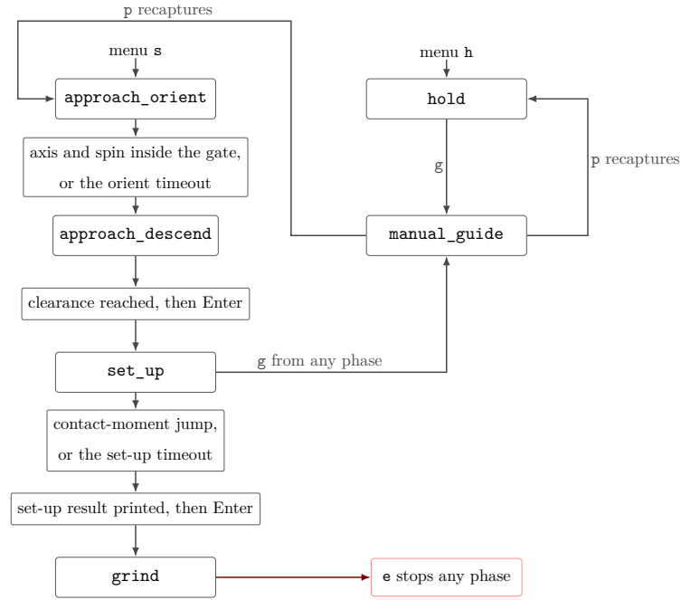
Figure 3.2: Run phase sequence and Cartesian pose hold.
