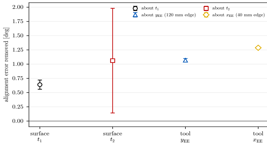
Figure 5.5: Case-E alignment improvement for surface-tangent and grinding-face-axis tilts.
