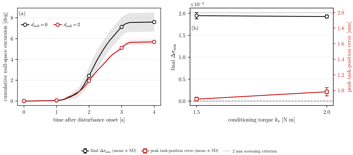
Figure 5.10: Null-space response during the Cartesian pose-hold disturbance test.
