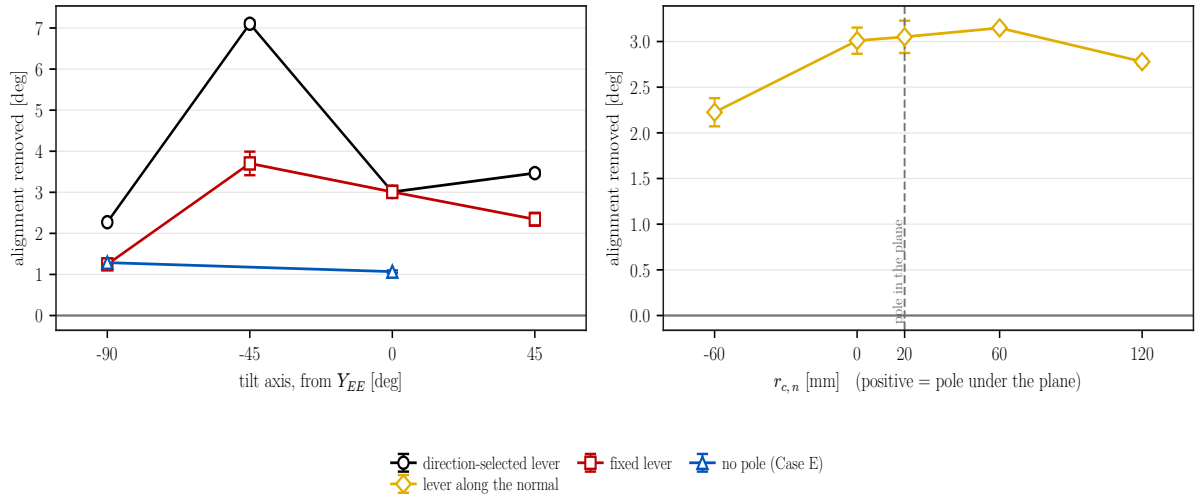
Figure 5.9: Alignment response by tilt direction and by normal lever coordinate.
