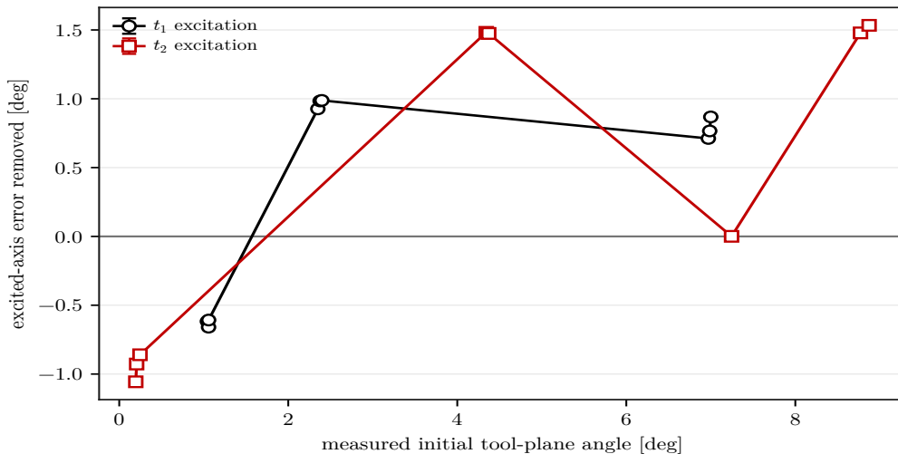
Figure 5.1: Case-A alignment improvement as a function of the measured initial alignment angle.
