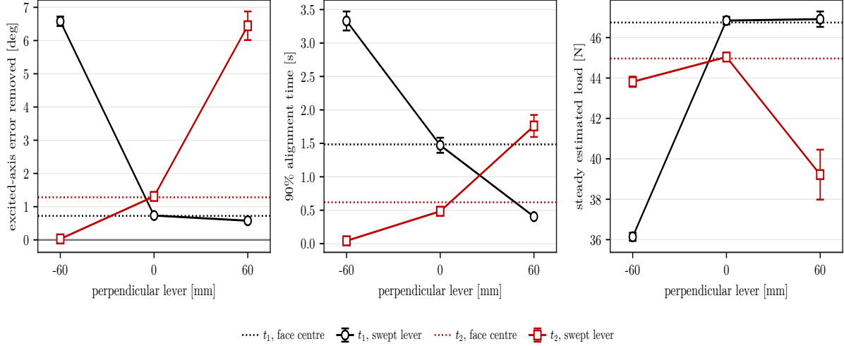
Figure 5.4: Case-D alignment response for the tested compliance-centre levers.
