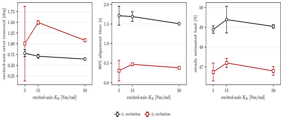
Figure 5.2: Case-B alignment improvement for the tested tilted-axis rotational stiffnesses.
