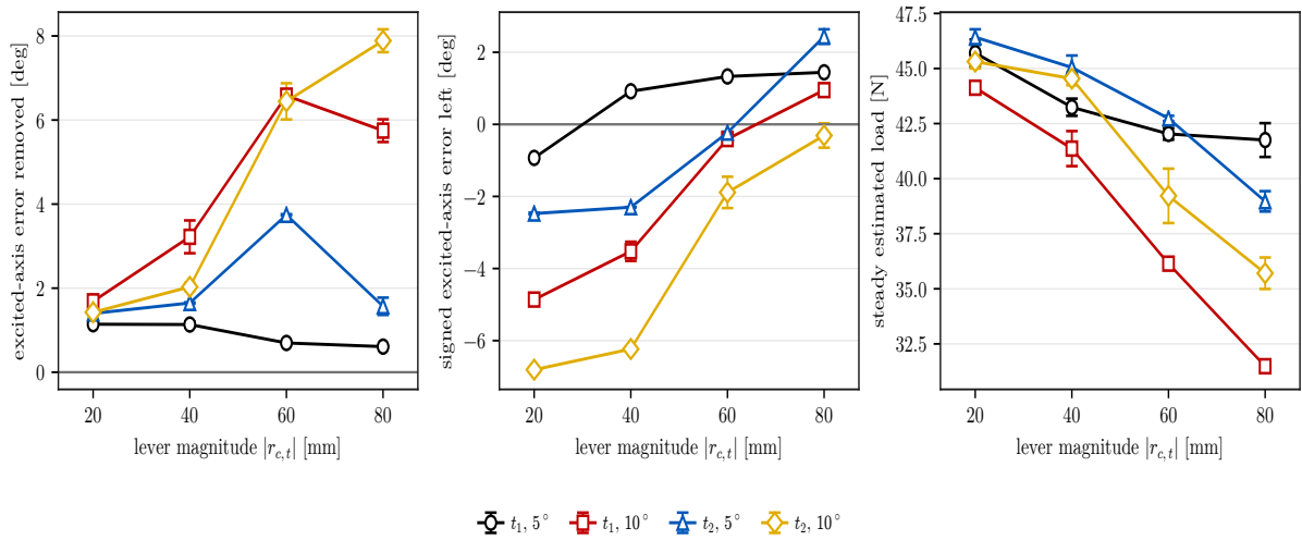
Figure 5.8: Alignment improvement, residual angle, and load by lever magnitude.
