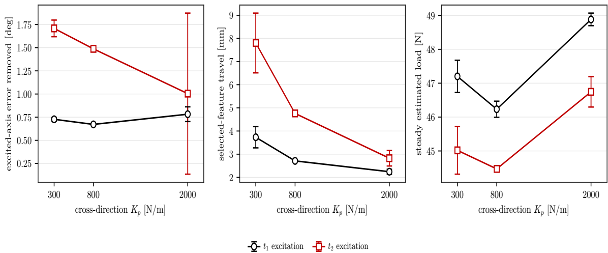
Figure 5.3: Case-C alignment improvement for the tested perpendicular translational stiffnesses.
