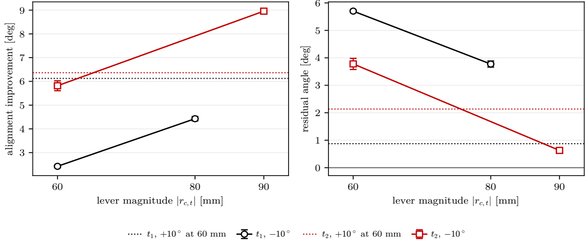
Figure 5.7: Reversed-tilt response at the extended lever magnitudes.
