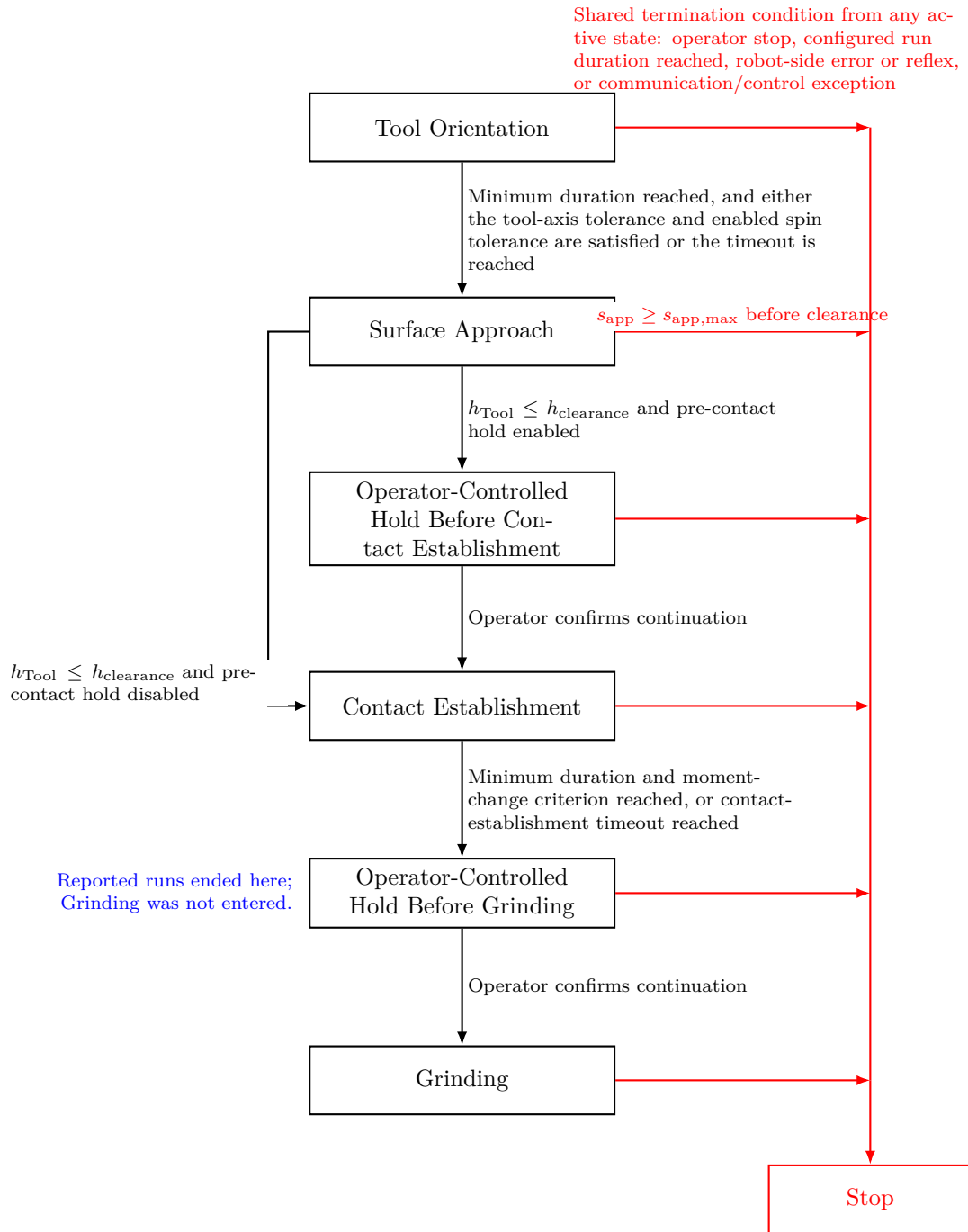
Figure 3.3: Surface-contact state transitions.
