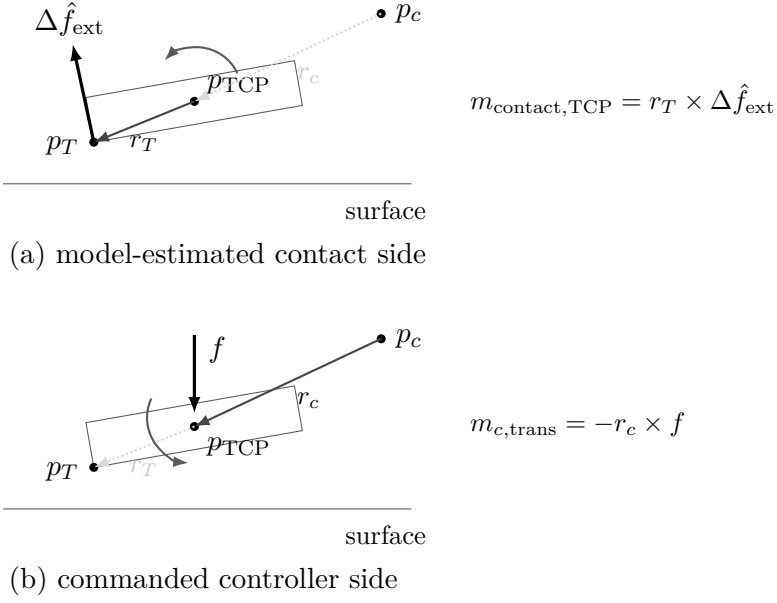
Figure 2.2: Which lever pairs with which force to give which moment.
