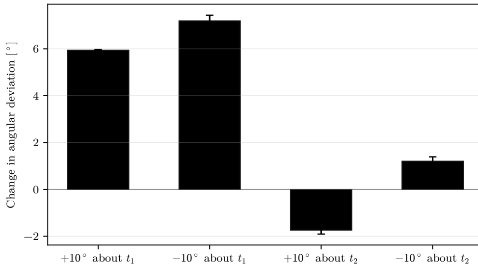
Figure 5.4: Alignment change with the centre of compliance on the TCP, by commanded offset.
