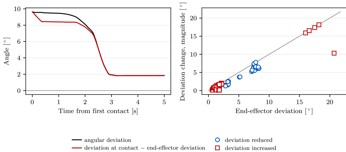
Figure 5.11: Agreement between the reported angular deviation and the rotation measured from joint angles alone.
