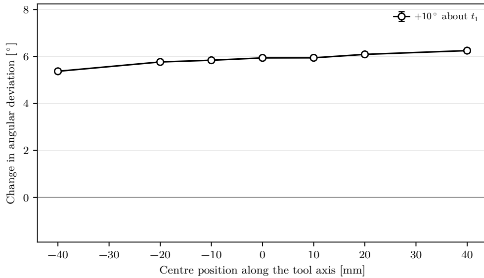
Figure 5.8: Alignment change by centre position along the tool axis.
