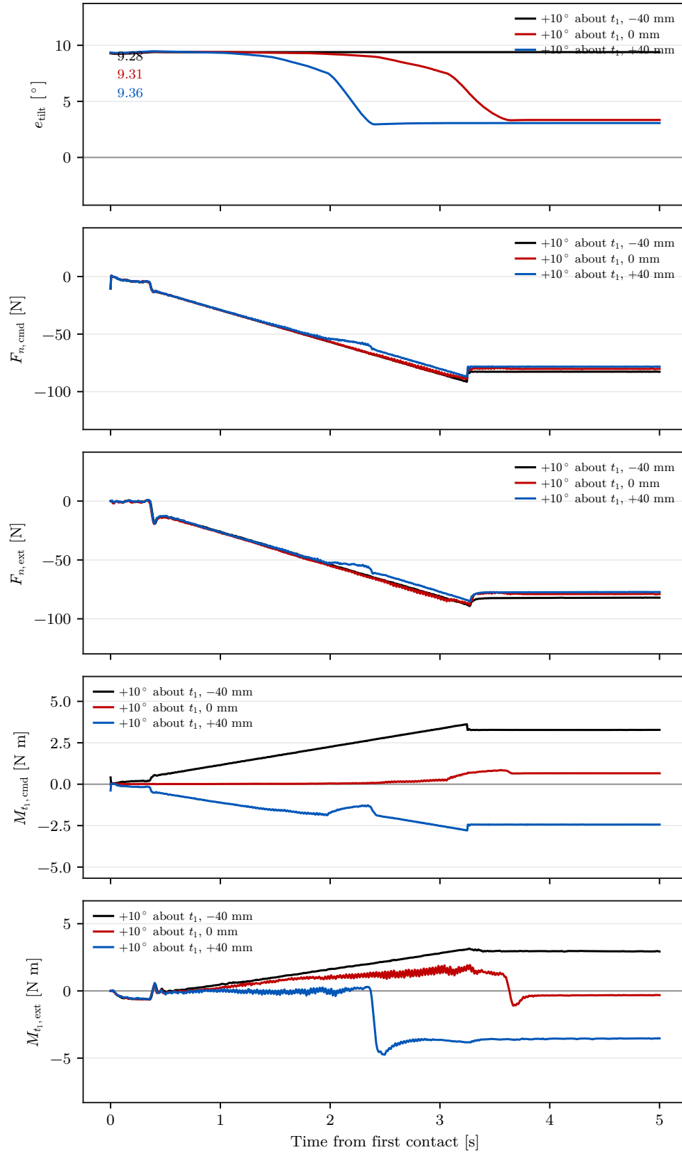
Figure 5.6: Deviation, normal press F_n and moment M_{t_1} for three centre positions, each commanded and model-estimated. All three carry a commanded offset of +10^\circ about t_1 ; the deviation each arrived with is printed beside the start of its curve.
