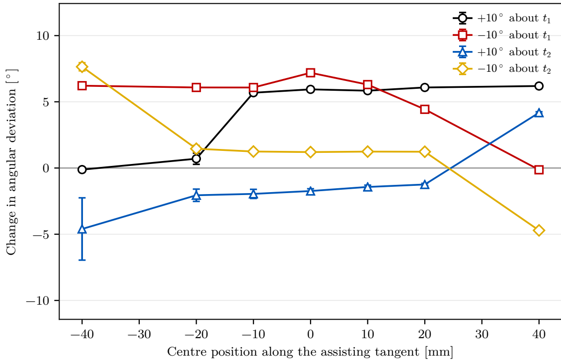
Figure 5.5: Alignment change by centre position along the assisting tangent, for both surface tangents and both signs of the commanded offset.
