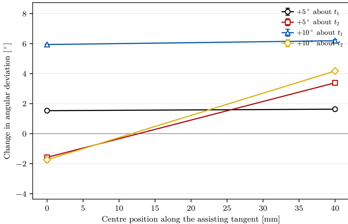
Figure 5.9: Alignment change at both commanded magnitudes, by centre position along the assisting tangent.
