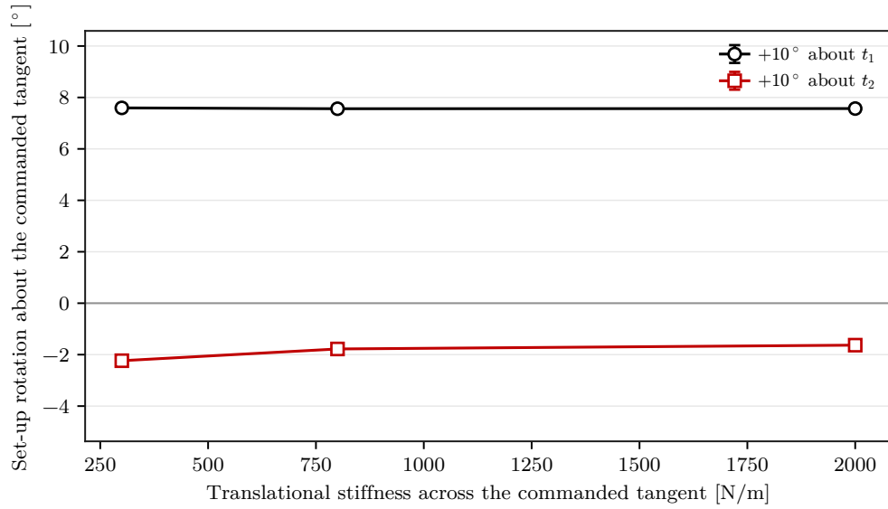
Figure 5.3: Set-up rotation about the commanded tangent by translational stiffness across it.
