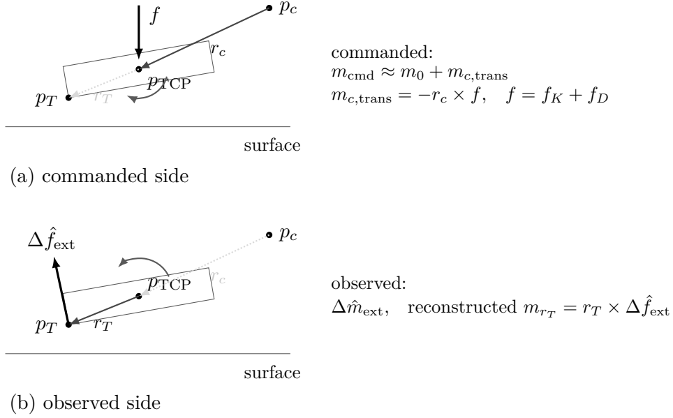
Figure 2.2: Which lever pairs with which force to give which moment.
