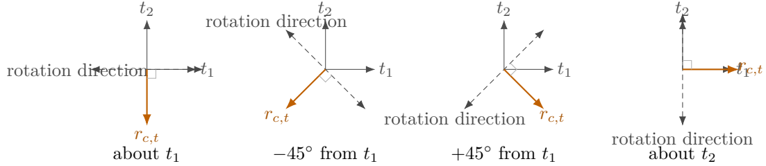
Figure 4.4: Selected tangential lever for each commanded rotation direction.
