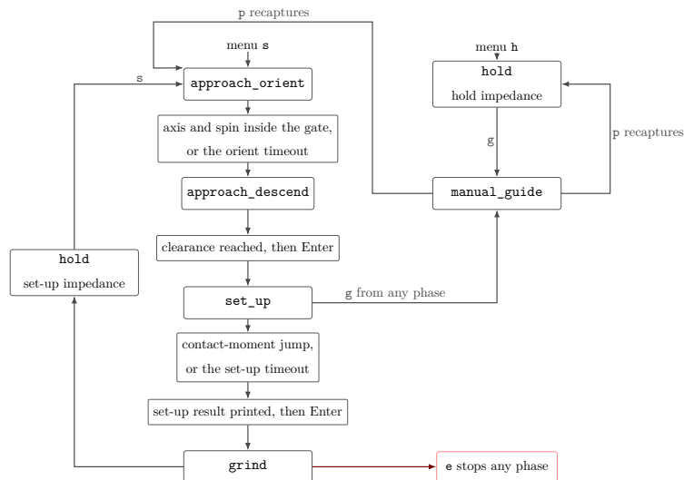
Figure 3.2: Run phase sequence and Cartesian pose hold.
