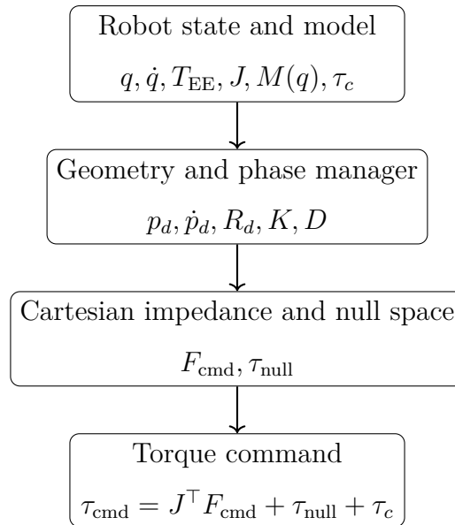
Figure 3.1: Real-time controller data flow.
