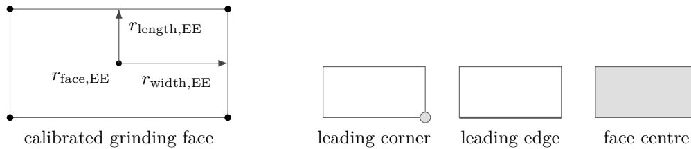
Figure 3.2: Grinding-face geometry and the selected leading feature.
