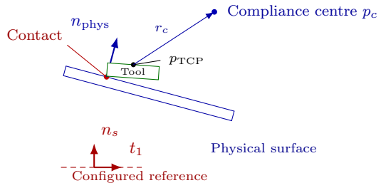
(b) Contact geometry
