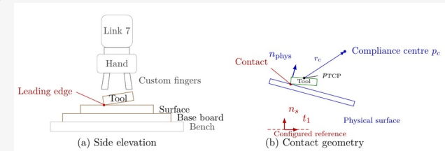
Figure 4.1: Experimental system: (a) physical set-up and (b) surface-frame contact geometry.
