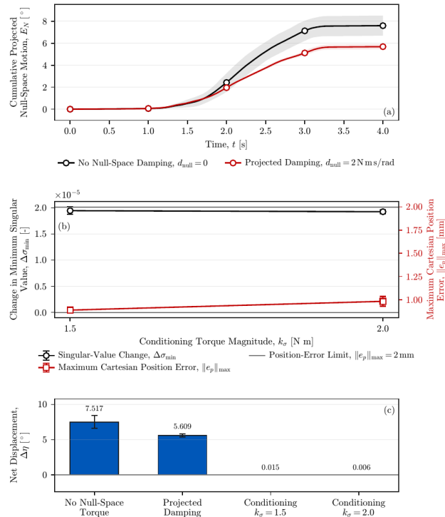
Figure 5.9: Null-space pose-hold response.
