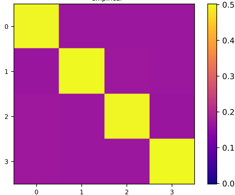
P_{\text{empirical}}
