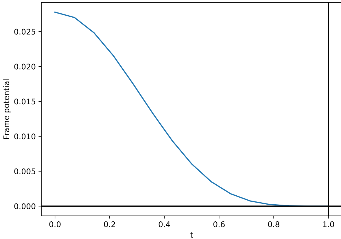
d = 2: Stabilizer to SIC state
