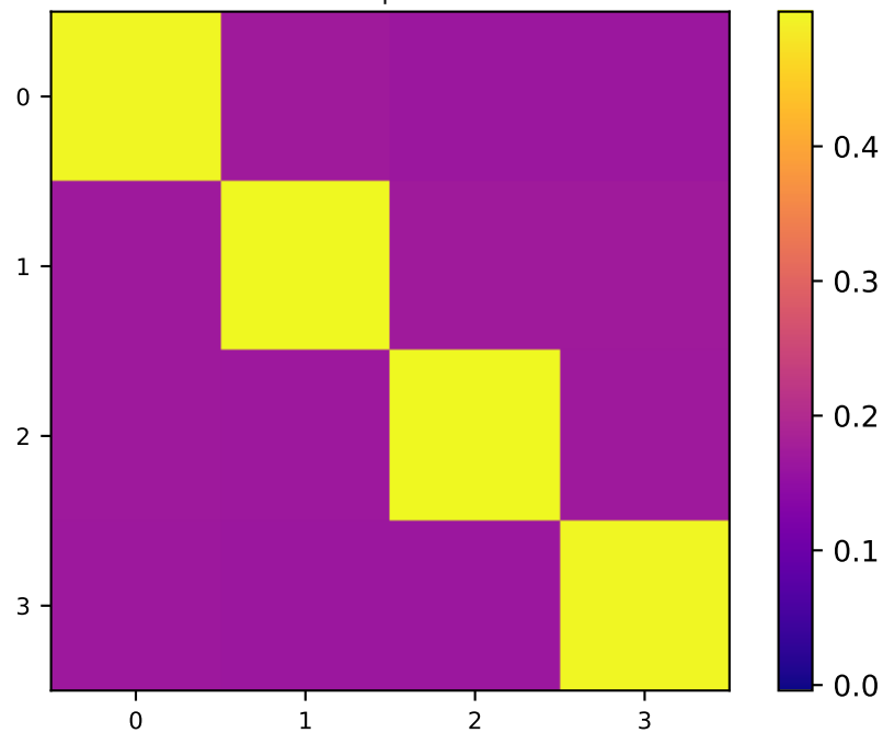
P_{\text{empirical}}
