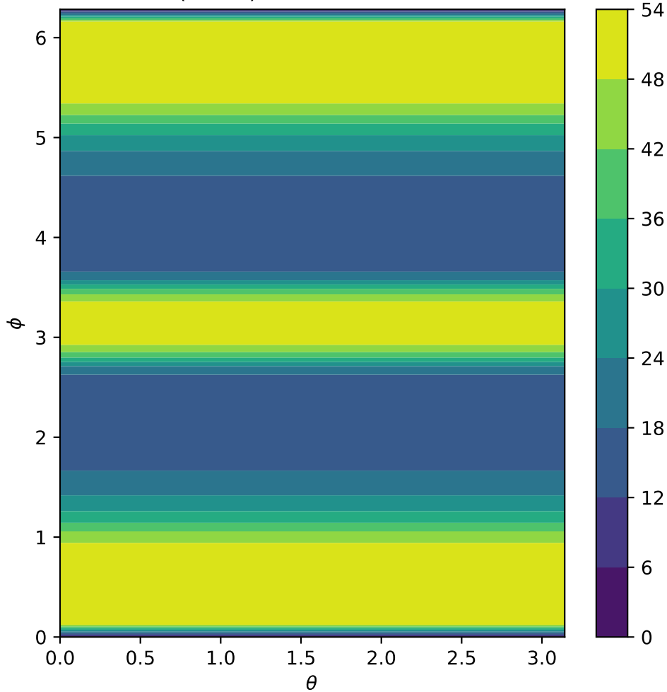
(Exact) LTP deformation
