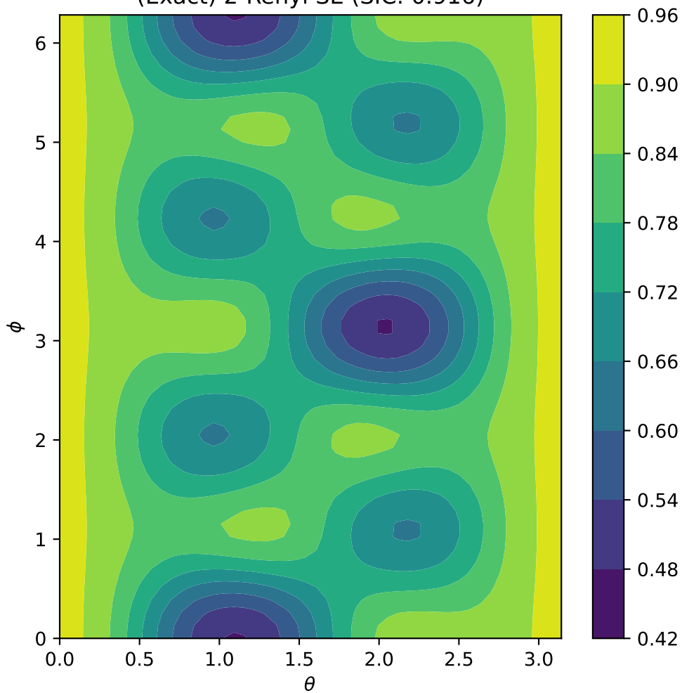
(Exact) 2-Renyi SE (SIC: 0.916)
