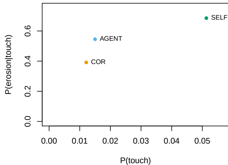
SELF REFLECT
