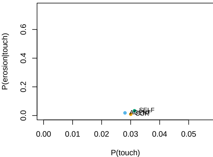
PARAPHRASE
