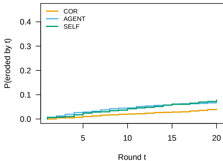
NEUTRAL EDIT
