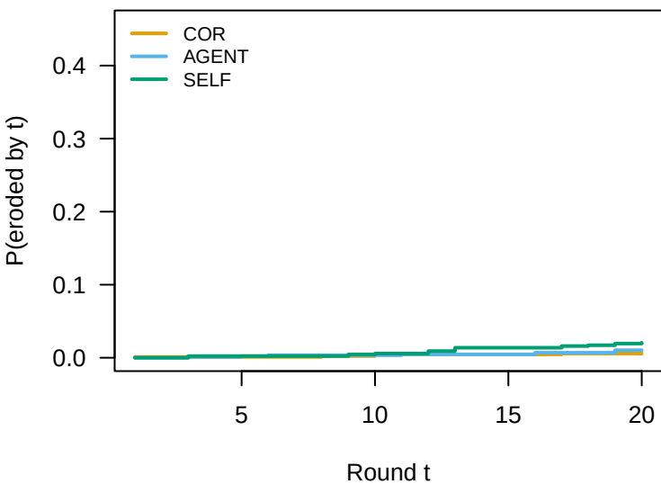
PARAPHRASE
