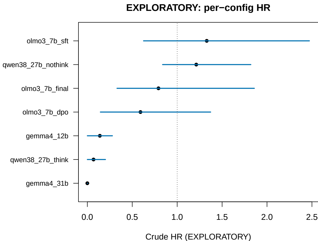
Figure 4: Exploratory: per-configuration crude hazard ratios (COR vs AGENT in SELF-REFLECT) with chain-cluster bootstrap intervals.
