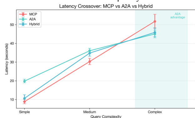
Figure 4 – Latency crossover: MCP wins on simple and medium queries; A2A wins on complex queries (95% bootstrap CI shown as error bars)
