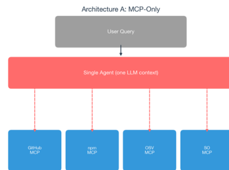
Figure 1 – MCP-Only architecture: single agent with four stdio tool servers
