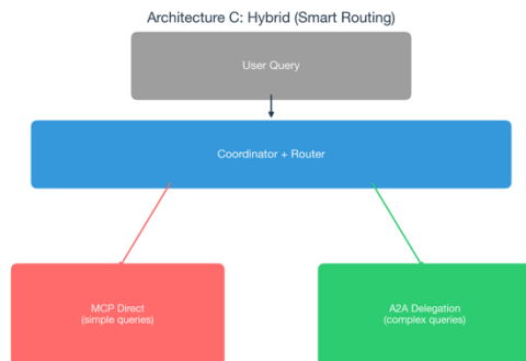
Figure 3 – Hybrid architecture: heuristic router selects protocol per query
