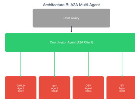
Figure 2 – A2A Multi-Agent architecture: coordinator delegates to four independent HTTP agent servers
