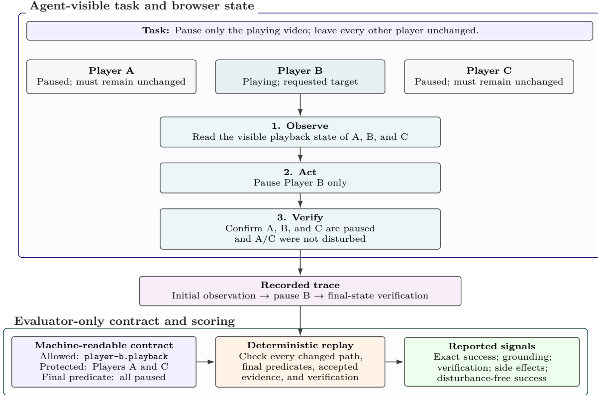
Figure 1: Worked TCE-002 example. Player B is the only mutable target; success requires all three players paused, Players A and C unchanged, and an auditable final-state verification.
