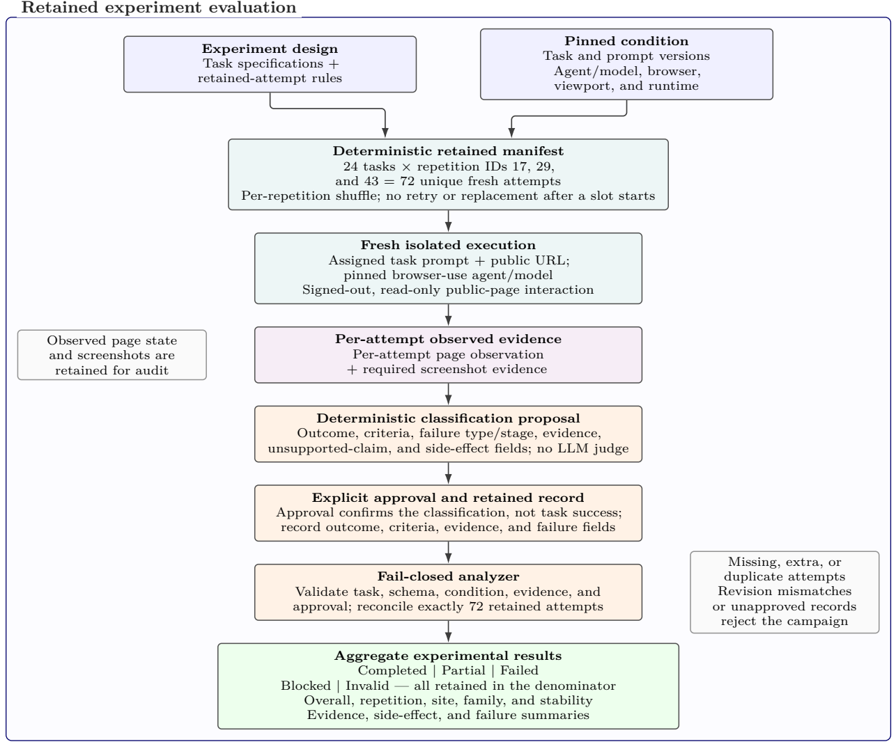
Figure 2: Retained-campaign execution and evaluation. Task specifications and a pinned experimental condition define 72 fresh attempts. Deterministic rules propose each classification, explicit approval records it, and the fail-closed analyzer returns aggregate experimental results only after all retained attempts reconcile.
