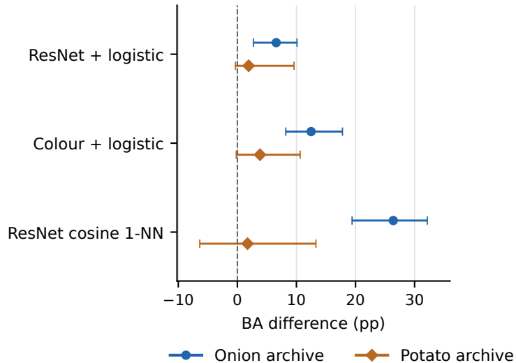
(a) Selected probes: exposure minus control BA
