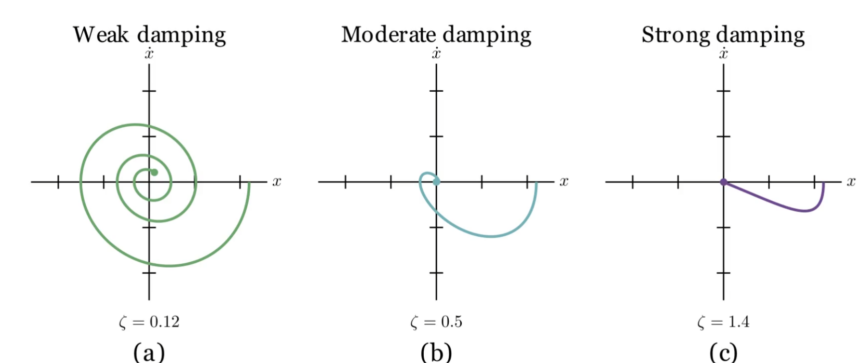
Figure: Phase-space trajectories for different damping regimes. In the weak damping regime ( \zeta = 0.12 ), the system exhibits oscillatory motion with a slowly decreasing amplitude, producing a spiral trajectory toward equilibrium. For moderate damping ( \zeta = 0.5 ), the oscillations decay more rapidly and the trajectory approaches equilibrium with fewer cycles. In the strong damping regime ( \zeta = 1.4 ), the system returns to equilibrium without oscillating, characterizing an overdamped response.
