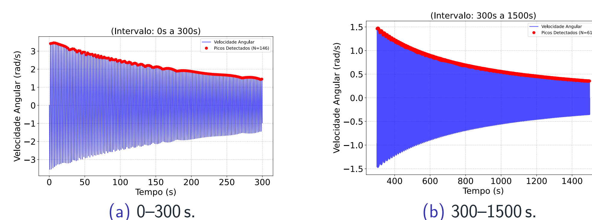
Figure: Velocity as a function of time for two different analysis intervals.
