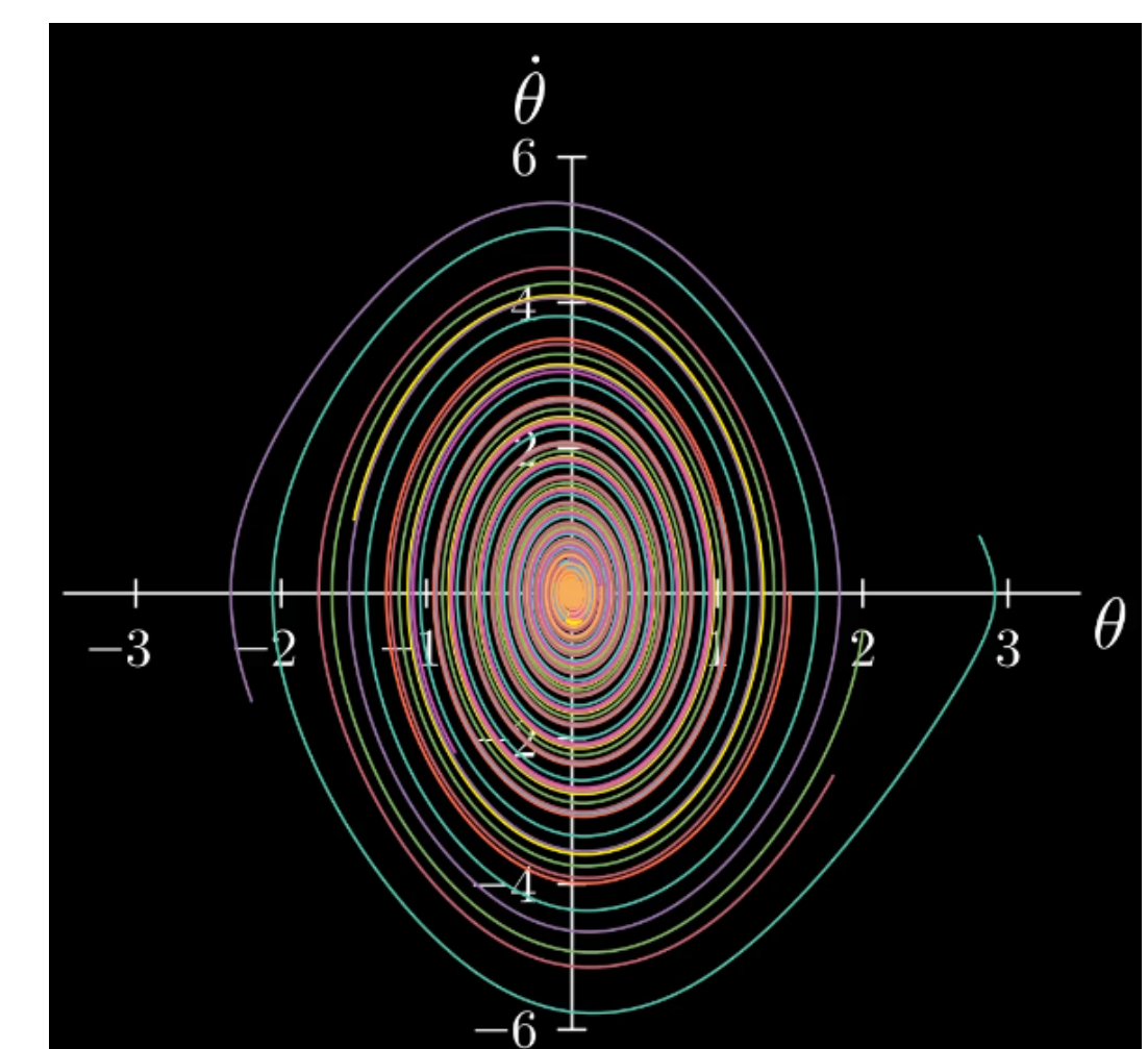
Figure: Phase-flow simulation with a set of 10 different initial conditions.
