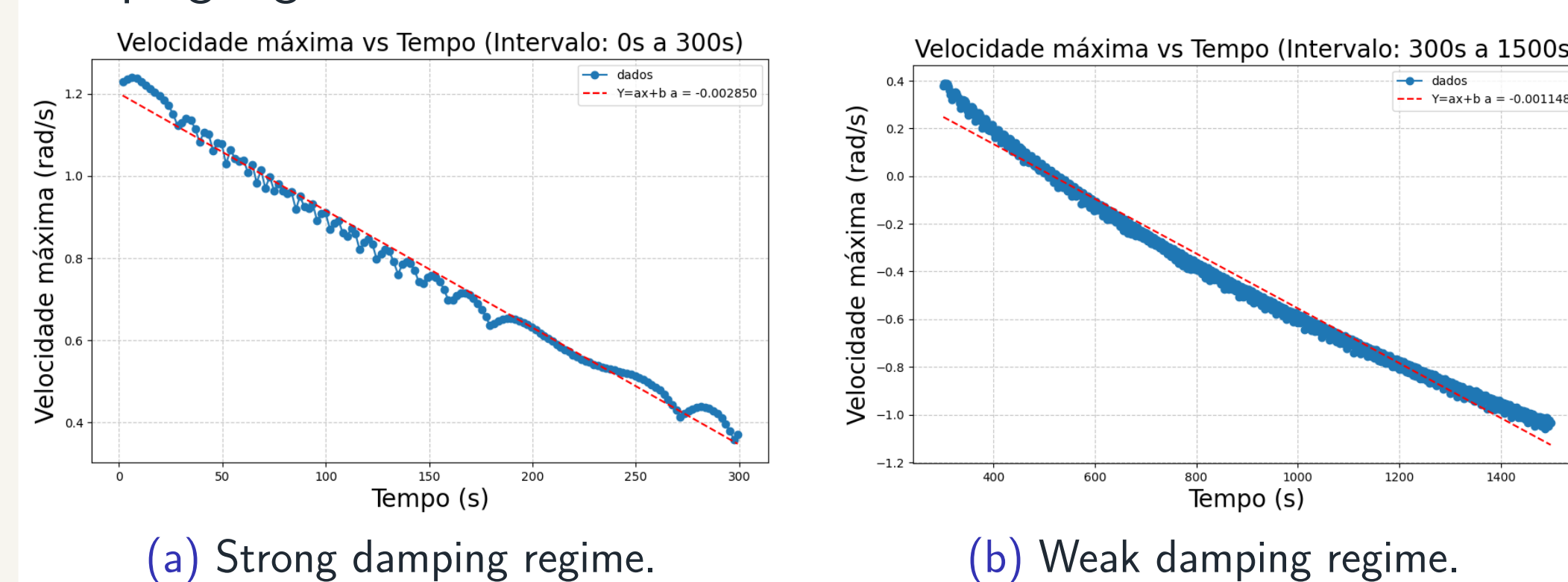
Figure: Maximum velocity as a function of time for two damping regimes.
