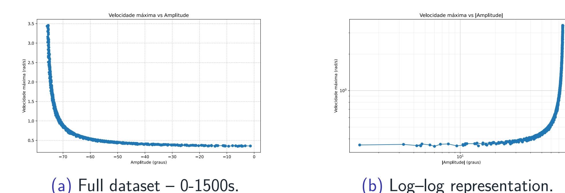
Figure: Maximum velocity as a function of amplitude.
