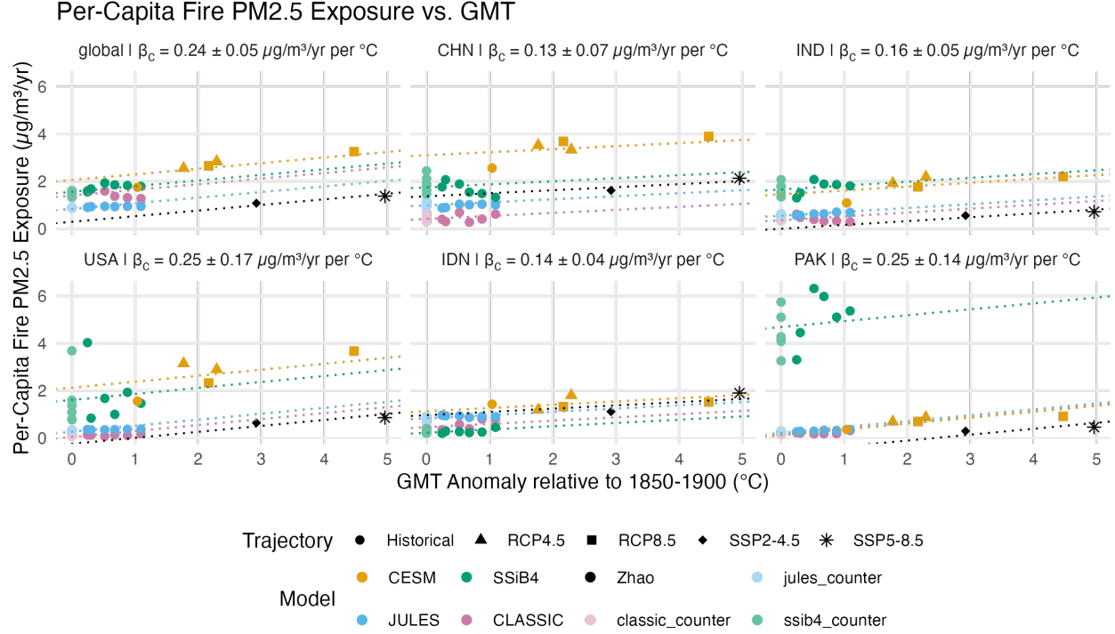
Figure 5: Per-capita wildfire PM2.5 exposure ( \mu\text{g}/\text{m}^3/\text{yr} ) by GMT change relative to the pre-industrial baseline ( ^\circ\text{C} ) for the five largest population countries as well as the global average. Each plot shows 43 observations from Park et al. (2024), Pierce et al. (2017), and Zhao et al. (2025). Point color indicates wildfire model; point shape indicates warming trajectory. The five dotted lines show the fitted line for each wildfire model, using the common slope \beta_c and the unique fixed-effect intercept.
