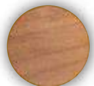
MOHO
