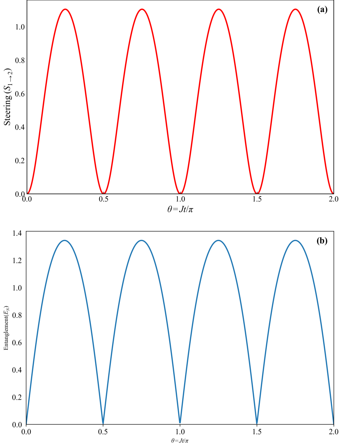
Figure 4.1: Two kinds of quantum correlations (a) quantum steering and (b) quantum entanglement are plotted against dimensionless interaction time, for fixed parameters \mu_1 = \mu_2 = \mu = 1 , \tau_1 = \tau_2 = \tau = 0.35 , \kappa_1 = \kappa_2 = \kappa = 0 and \phi_1 = 0 and \phi_2 = \pi/2 .
