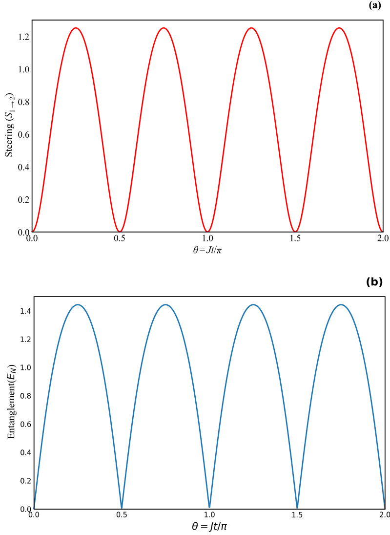
Fig4.3 Two kinds of quantum correlations: (a) quantum steering and (b) quantum entanglement are plotted against dimensionless interaction time, for fixed parameters \kappa_1 = \kappa_2 = \kappa = 0 and squeezing factor r = 0.5 .
