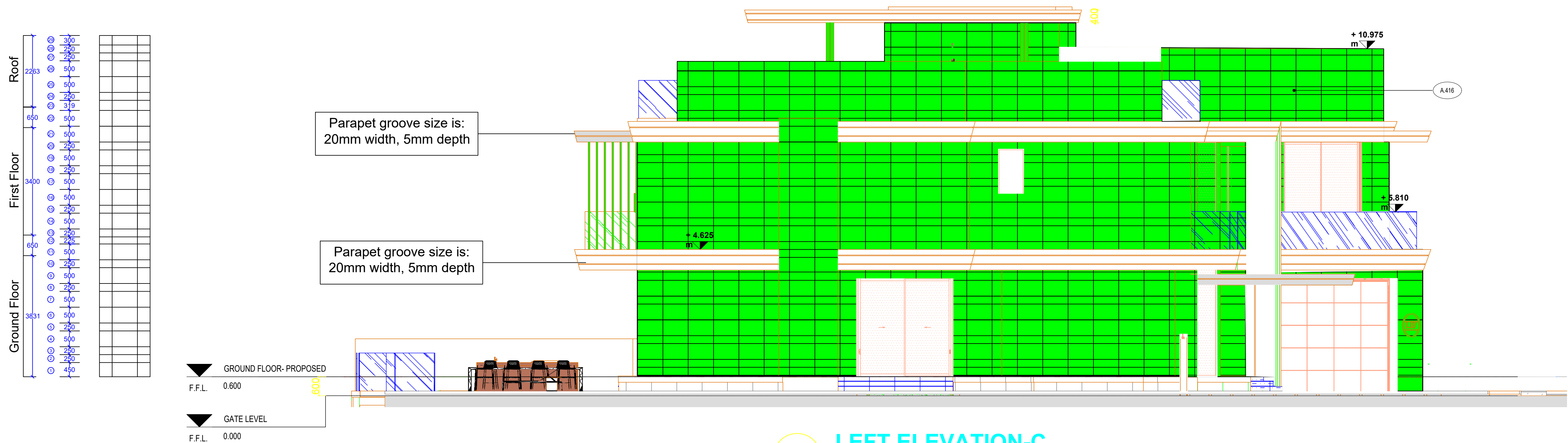
3 LEFT ELEVATION-C SCALE 1:100
