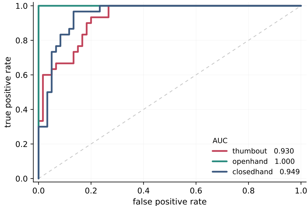
One-vs-rest ROC (90/90 hands localised at IoU \geq 0.5 )
