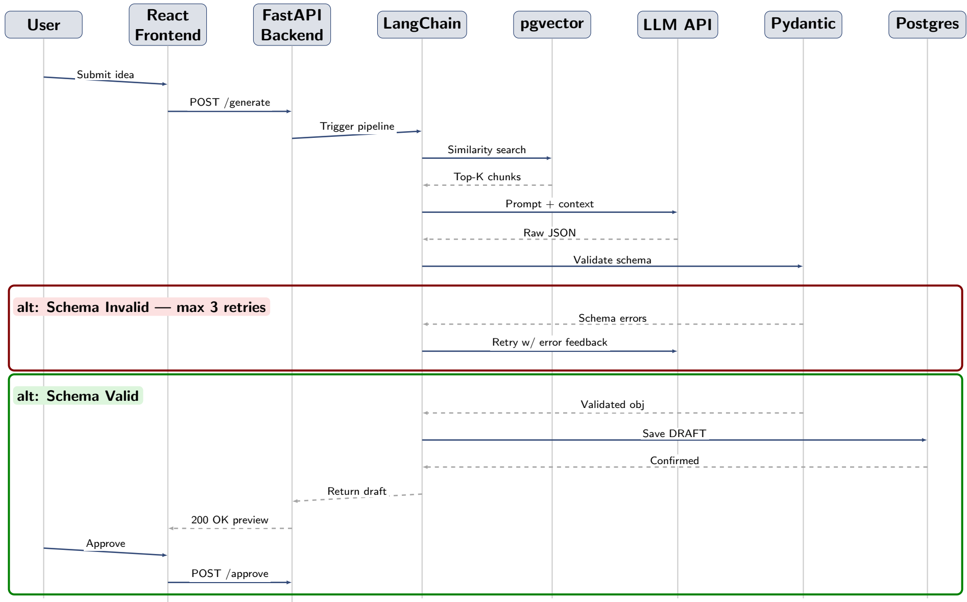
Figure 4: Sequence Diagram — Complete Pipeline
