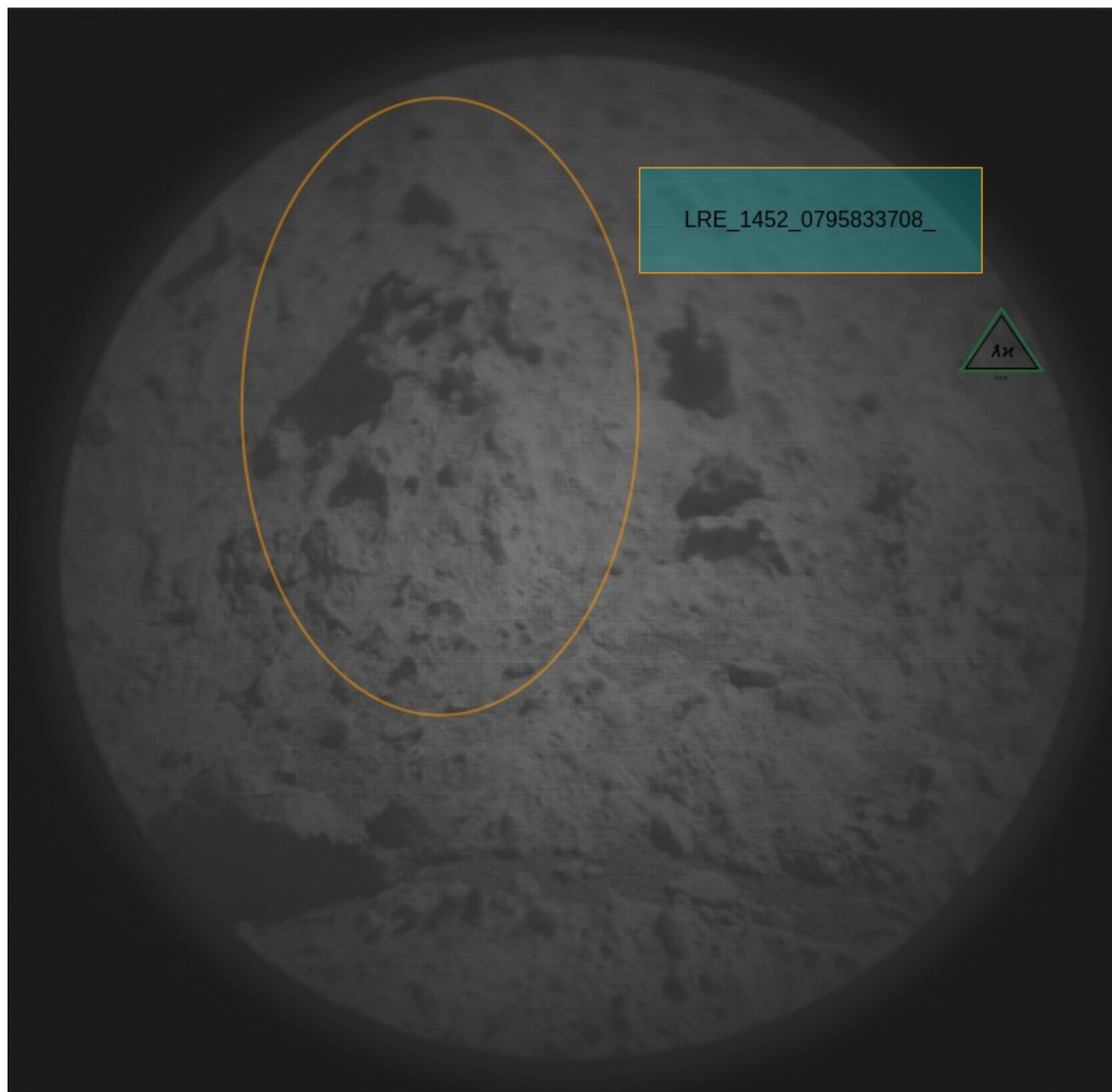
Figure 74: LRE_1452_0795833708_draw-23
