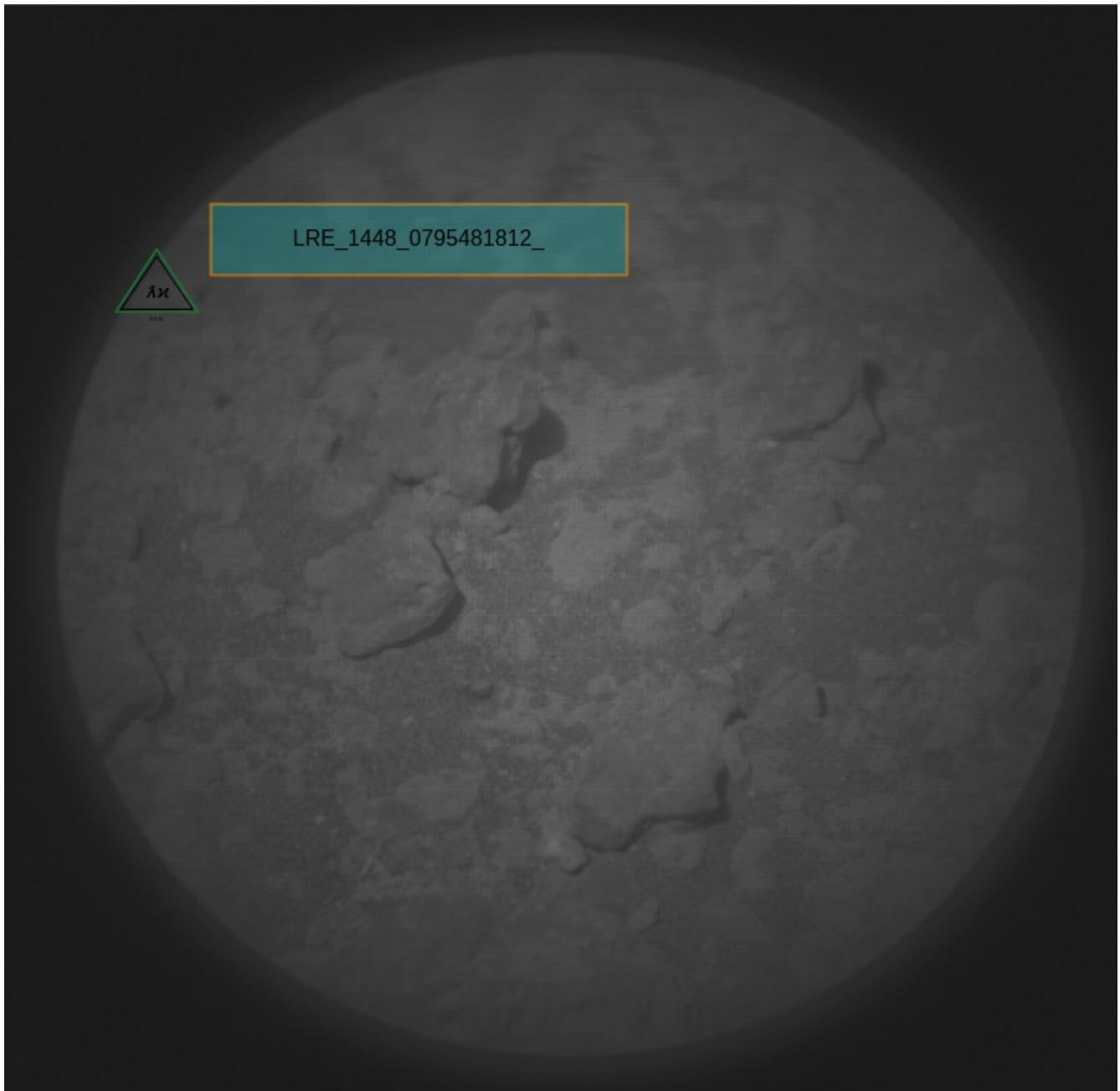
Figure 61: LRE_1448_0795481812_draw-21
