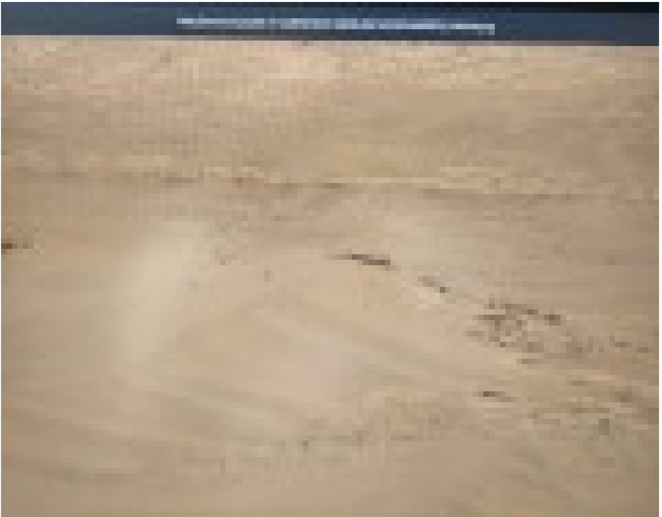
Figure 176: 1511_0670sanddunesovertile
