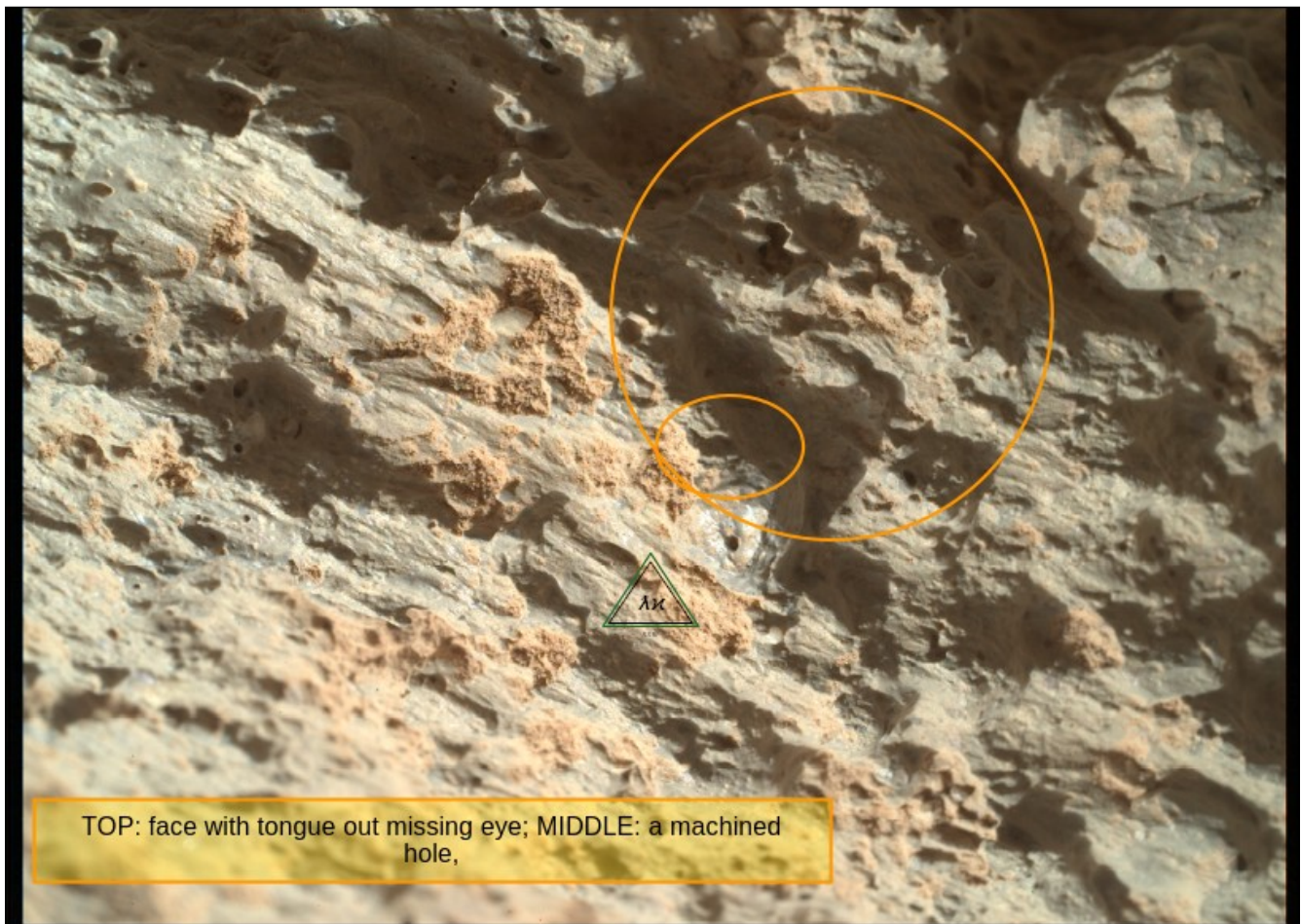
Figure 80: SIF_1453_0795942288_mod-212
