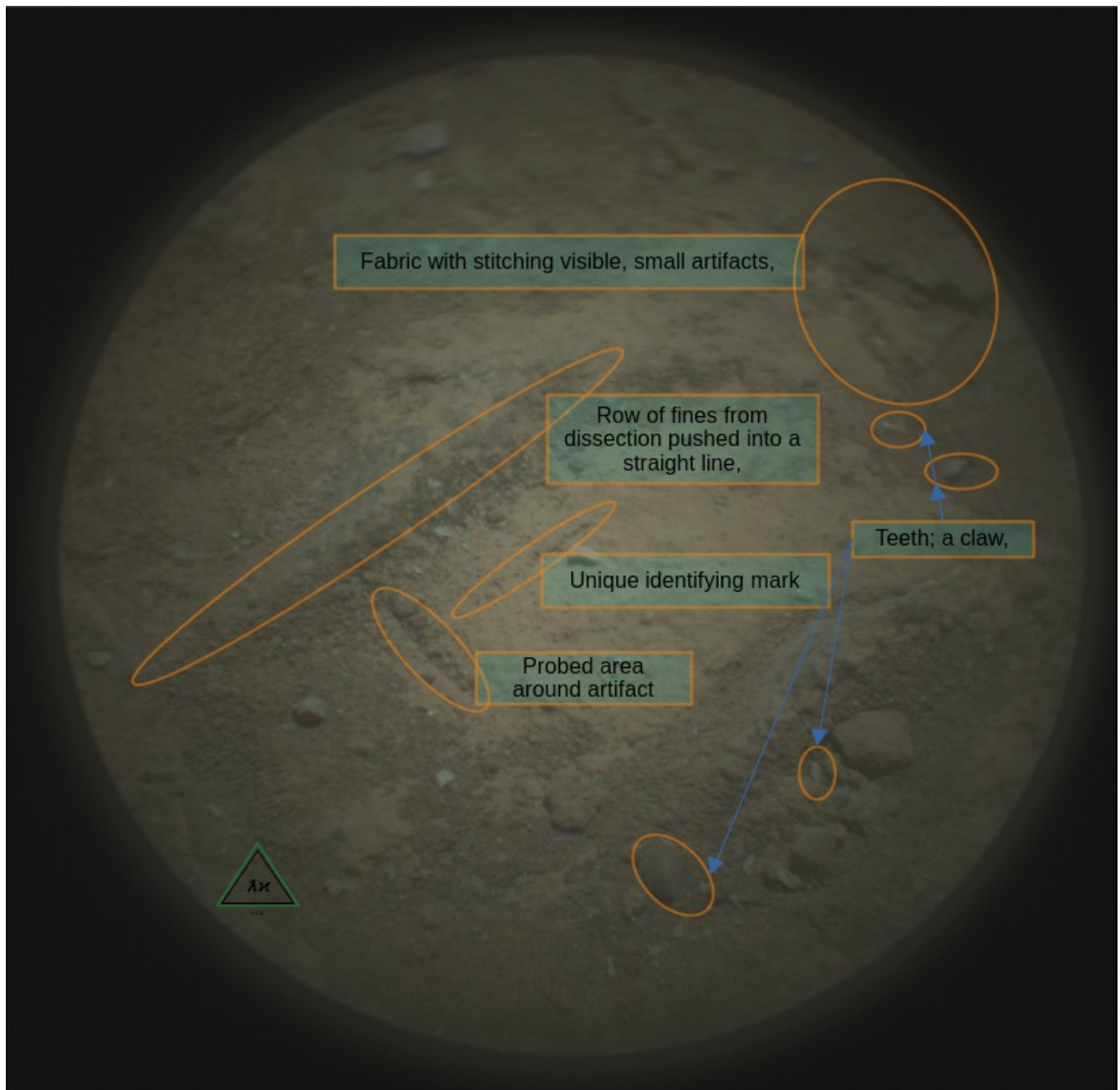
Figure 134: LRF_1480_0798330618_mod-235
