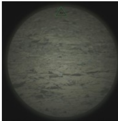
Figure 351434_1122
