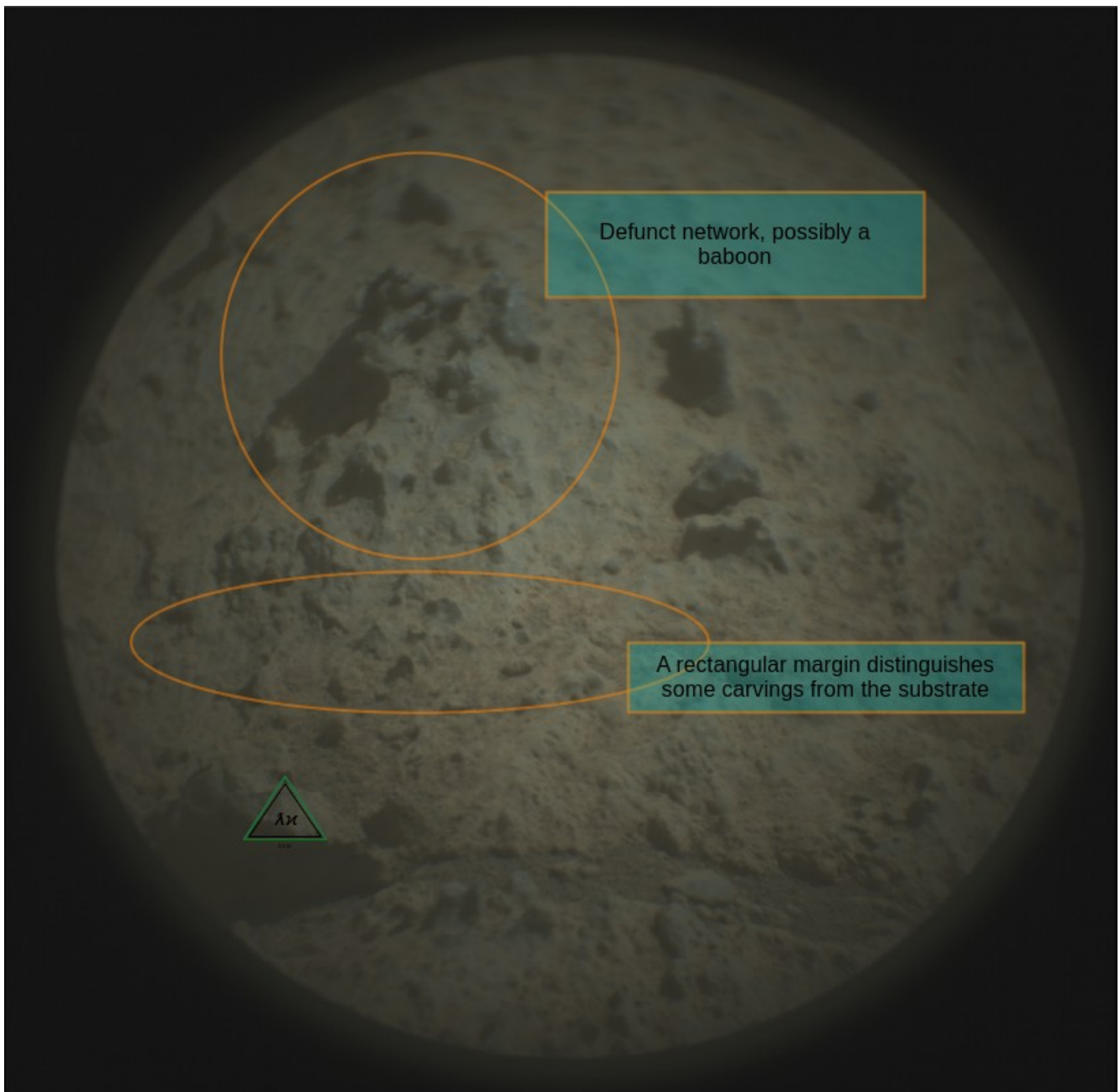
Figure 73: LRF_1452_0795833708_mod-209
