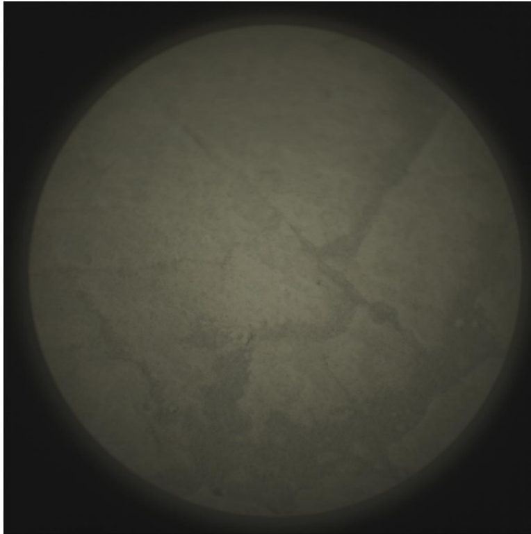
Figure 117: LRF_1470_0797429785_434EBY_N0710696SCAM01470_0 010I6J01_1200
