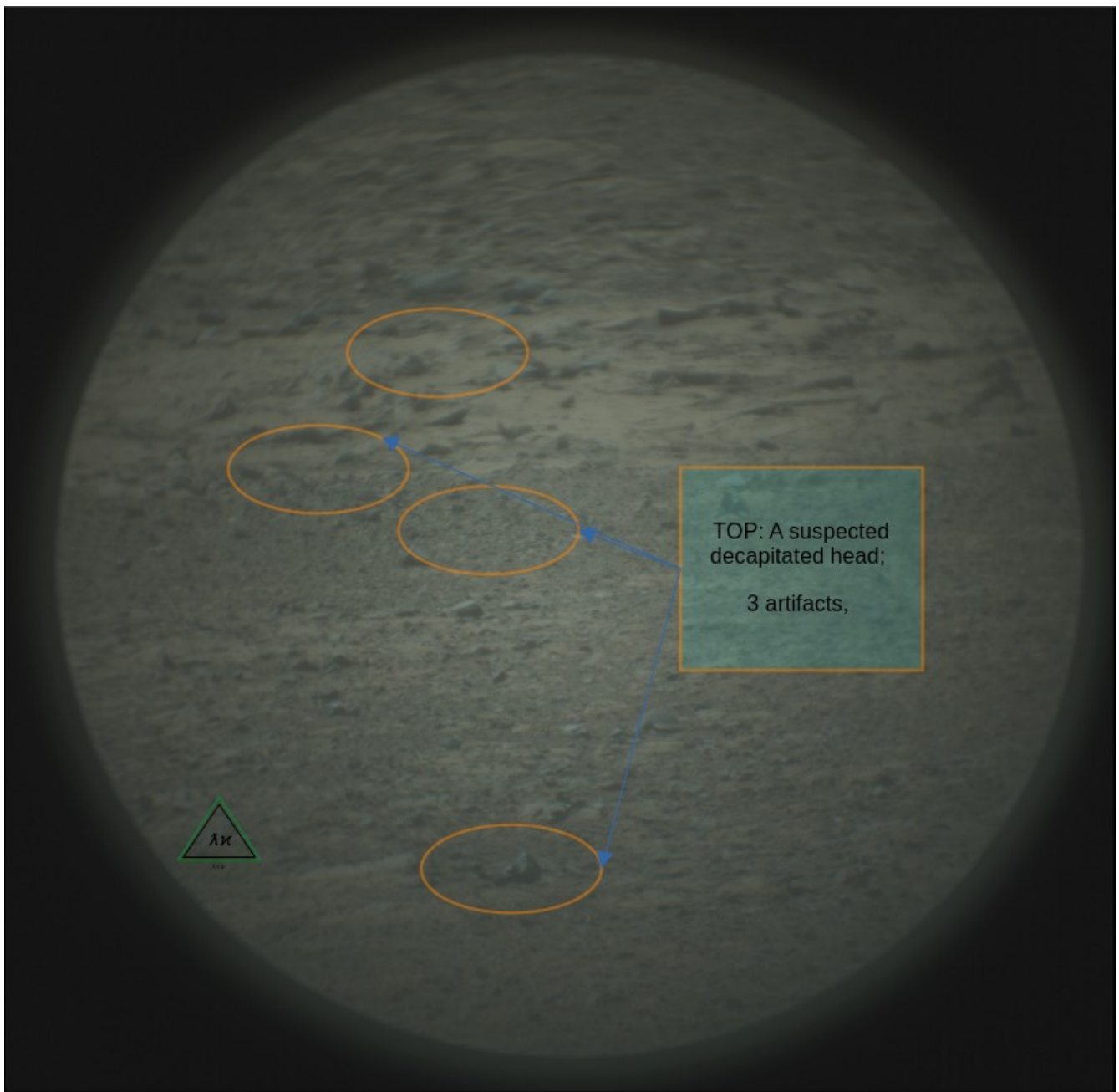
Figure 141: LRF_1486_0798853284_mod-238
