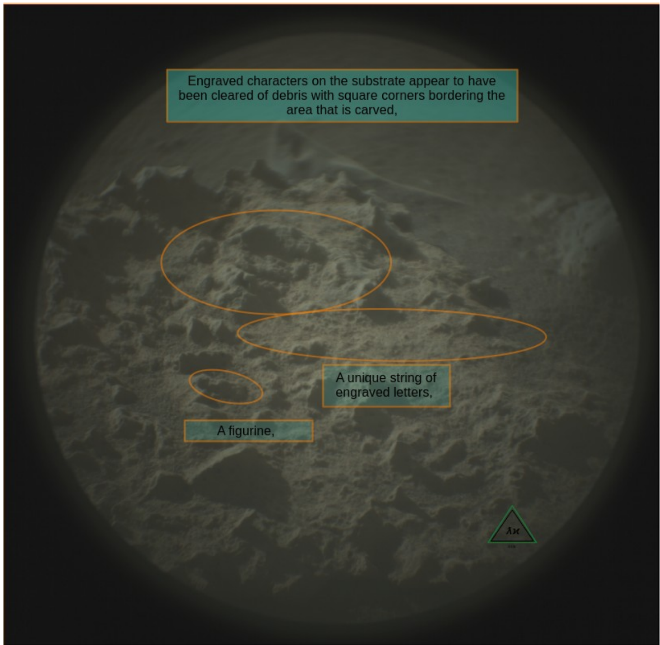
Figure 131: LRF_1478_0798135367_mod-232
