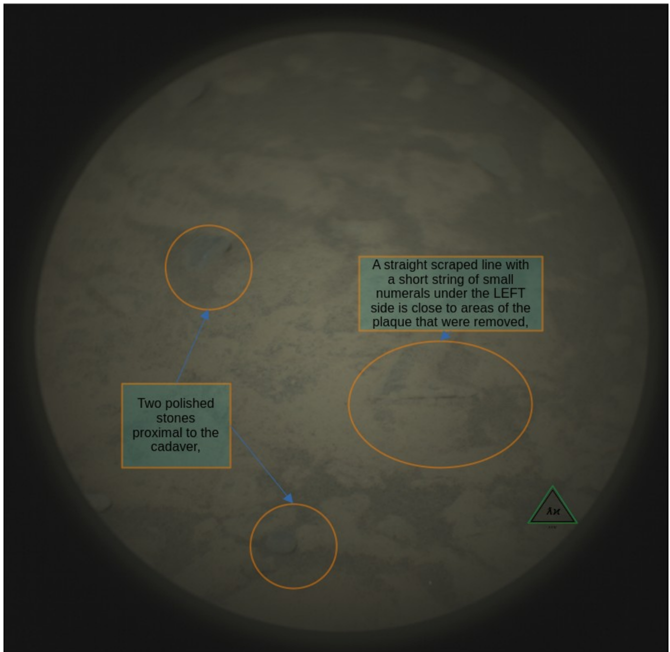
Figure 120: LRF_1473_0797698047_mod-230
