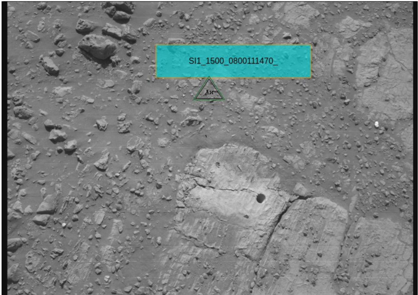
Figure 156: 1500_0800111470_draw-29
