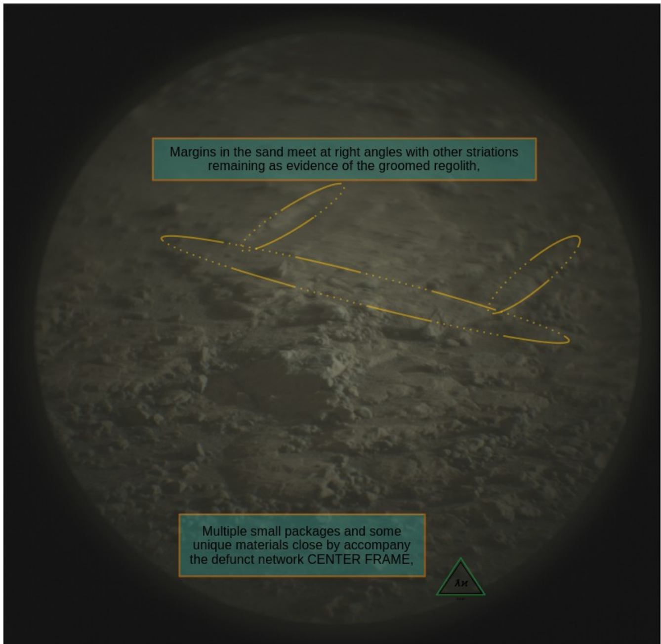
Figure 159: LRF_1503_0800349589_mod-241
