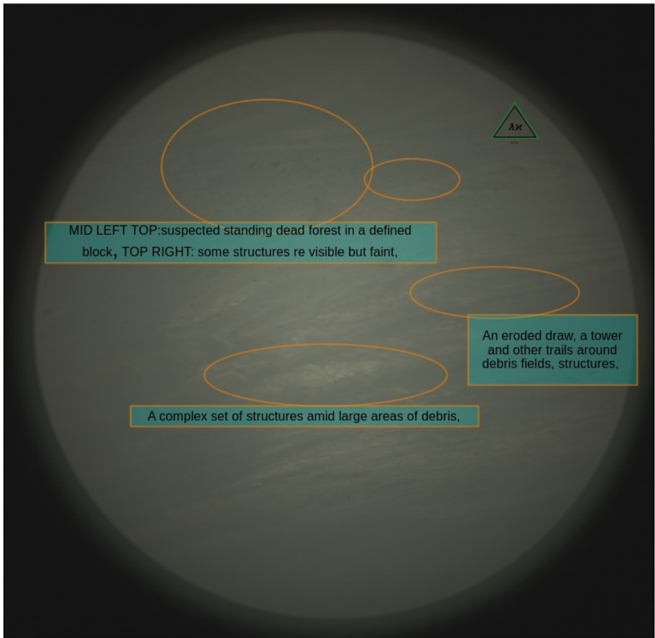
Figure 88: LRF_1458_0796368335_mod-216
