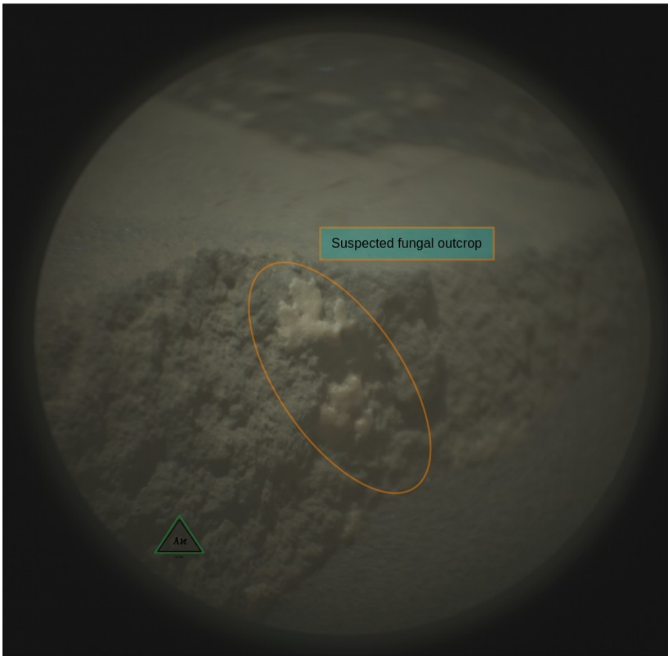
Figure 24: LRF_1426_0793528159_mod-194
