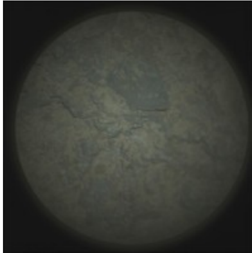
Figure 83: LRF_1457_0796278274_368EBY_N071 0056SCAM01457_0050I6J01_800
