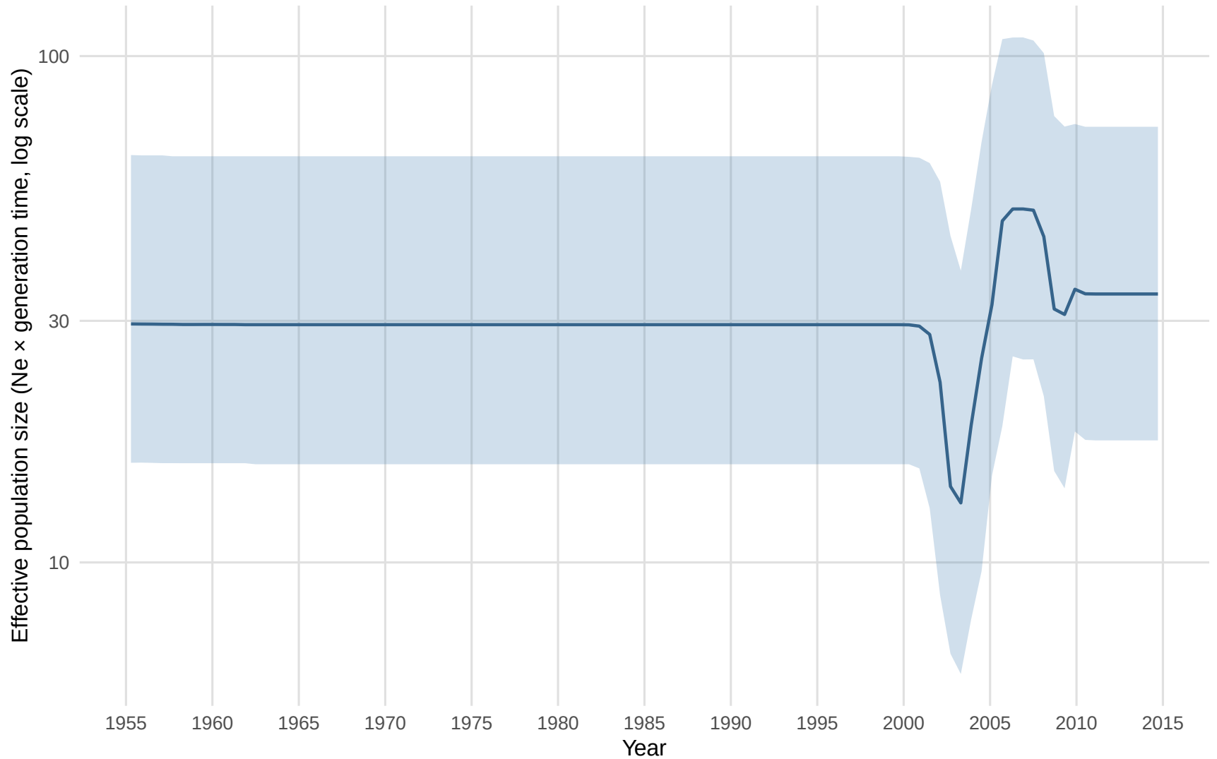
Bayesian Skyline Plot — Clade 2
