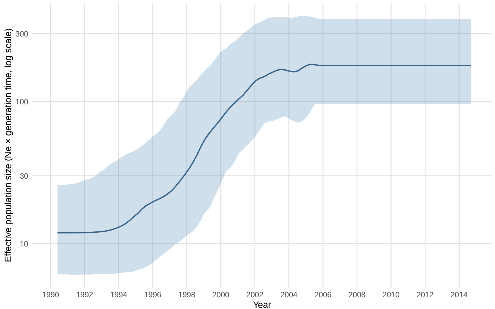
Bayesian Skyline Plot — Clade 1
