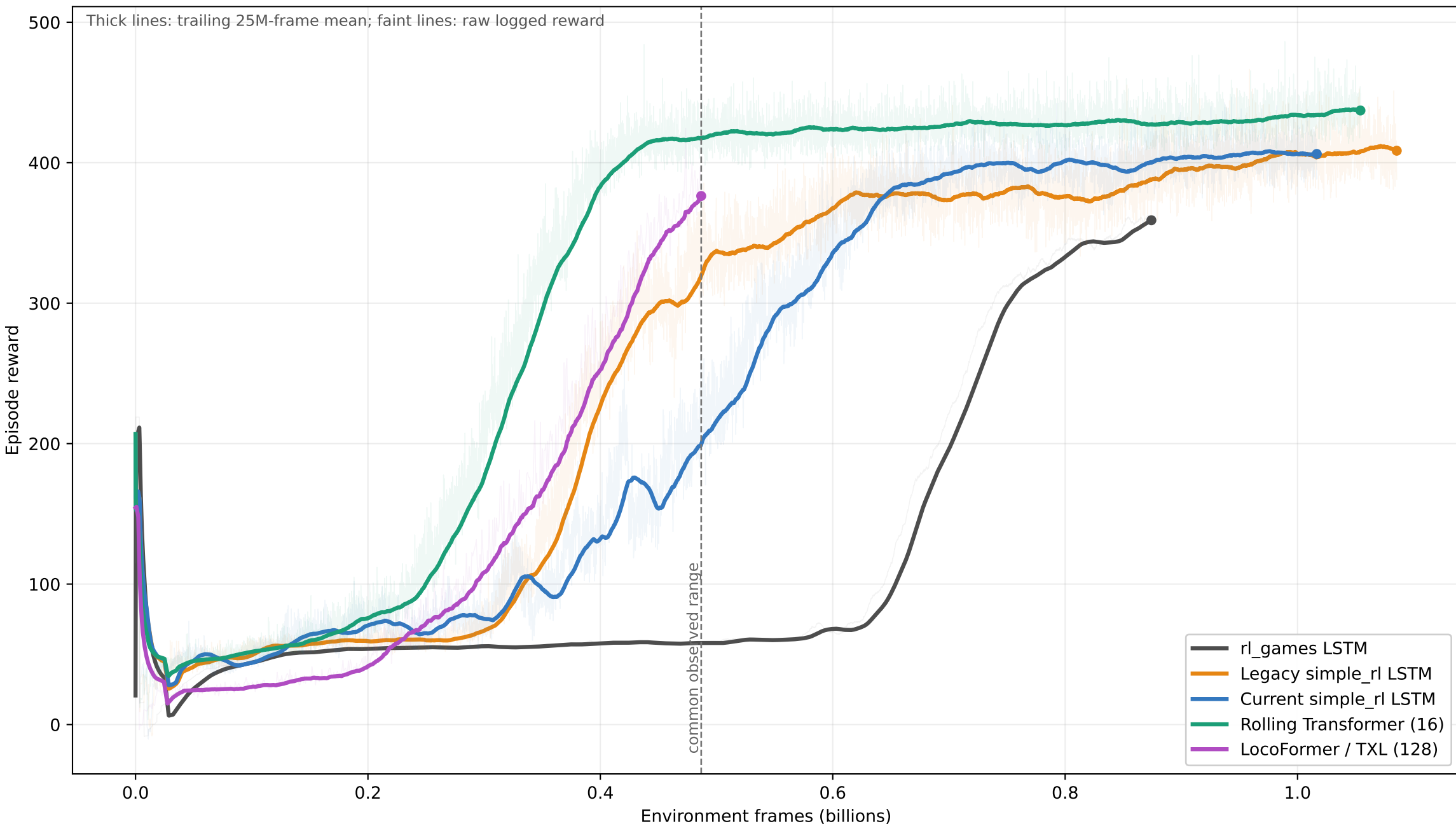
SimToolReal SAPG reward curves — seed 0
