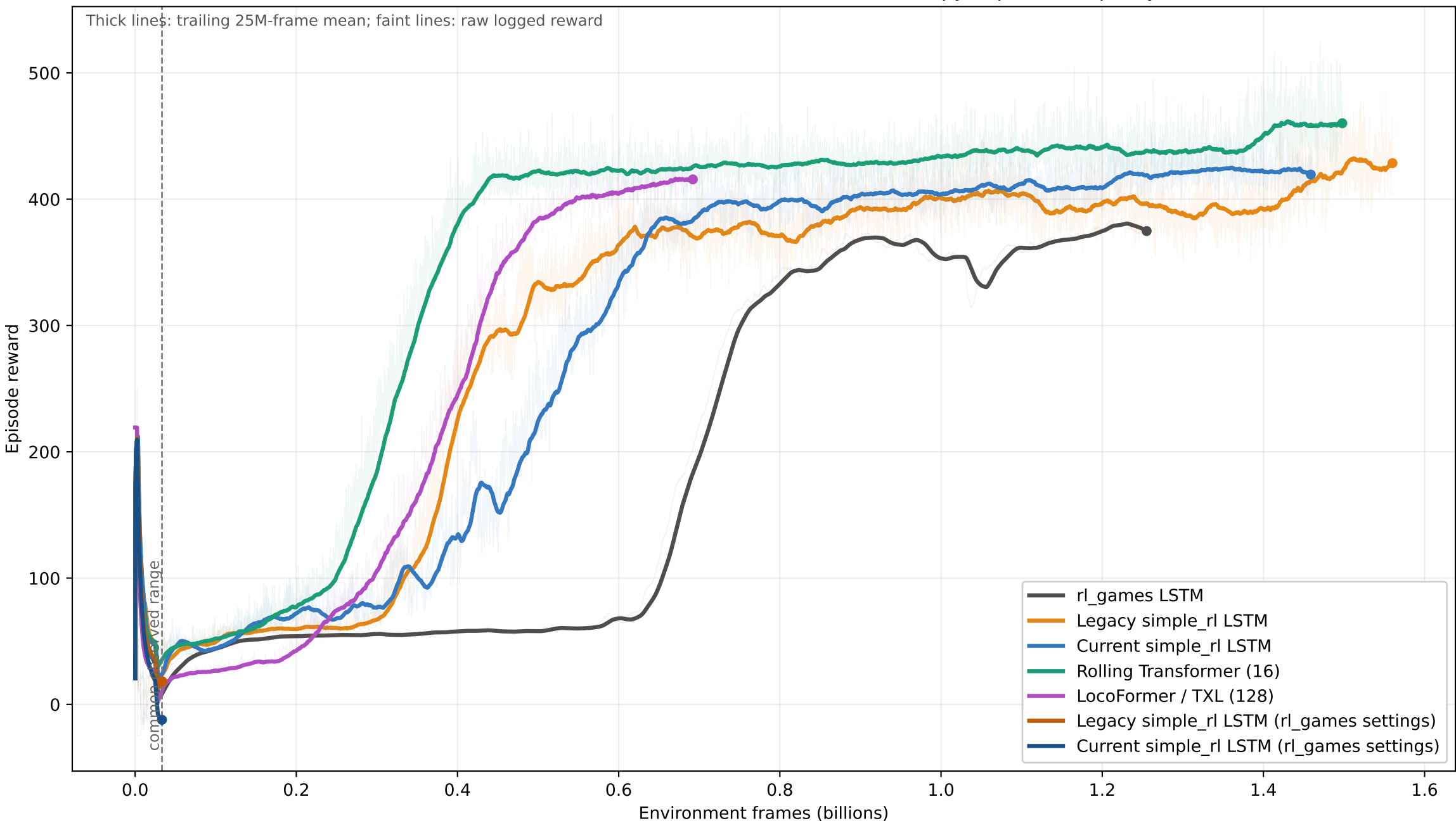
SimToolReal SAPG reward curves — seed 0 — zero-entropy exploitation policy
