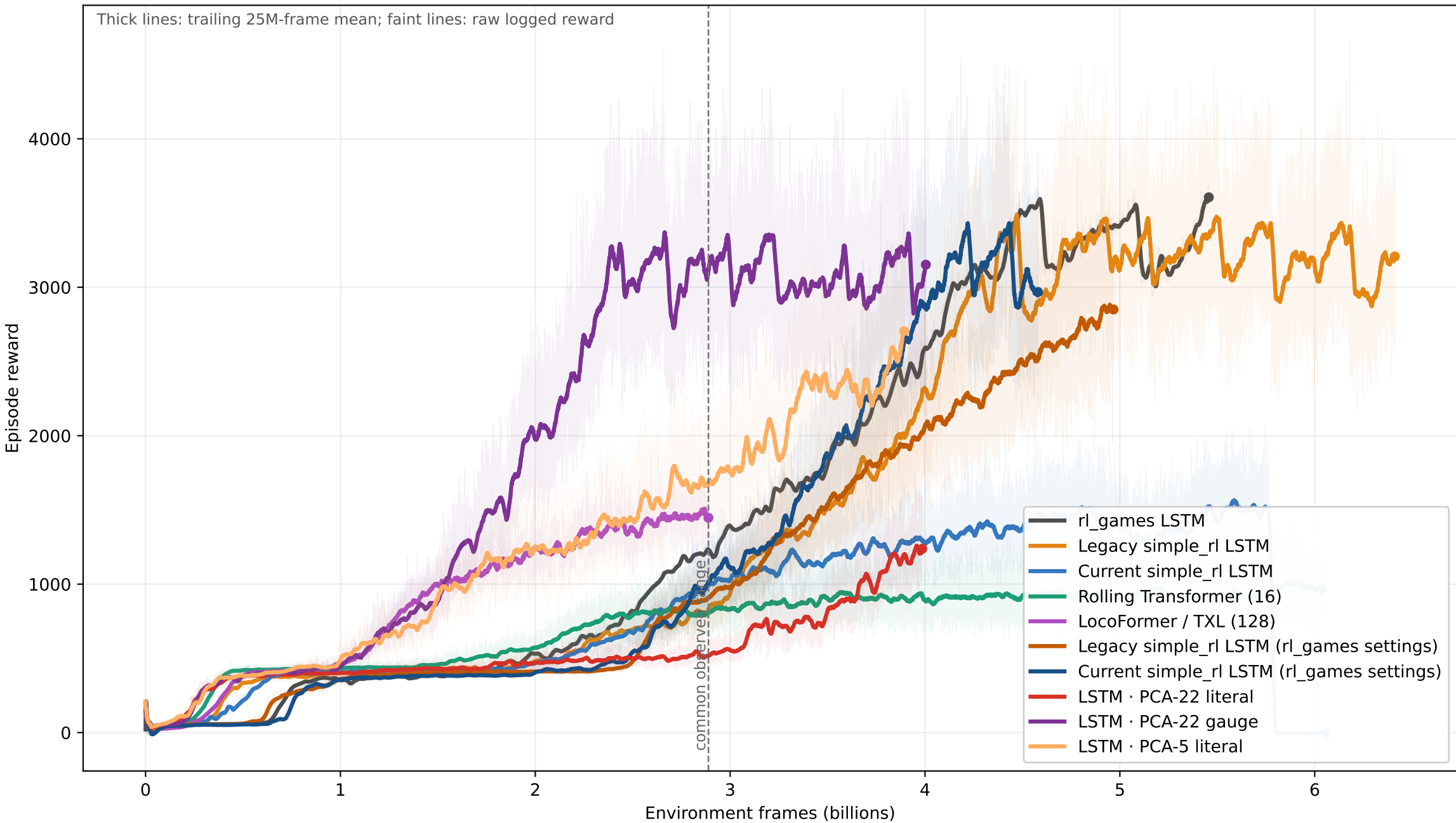
SimToolReal SAPG reward curves — seed 0 — all-policy aggregate
