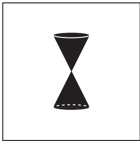
(3-1) General relativity
