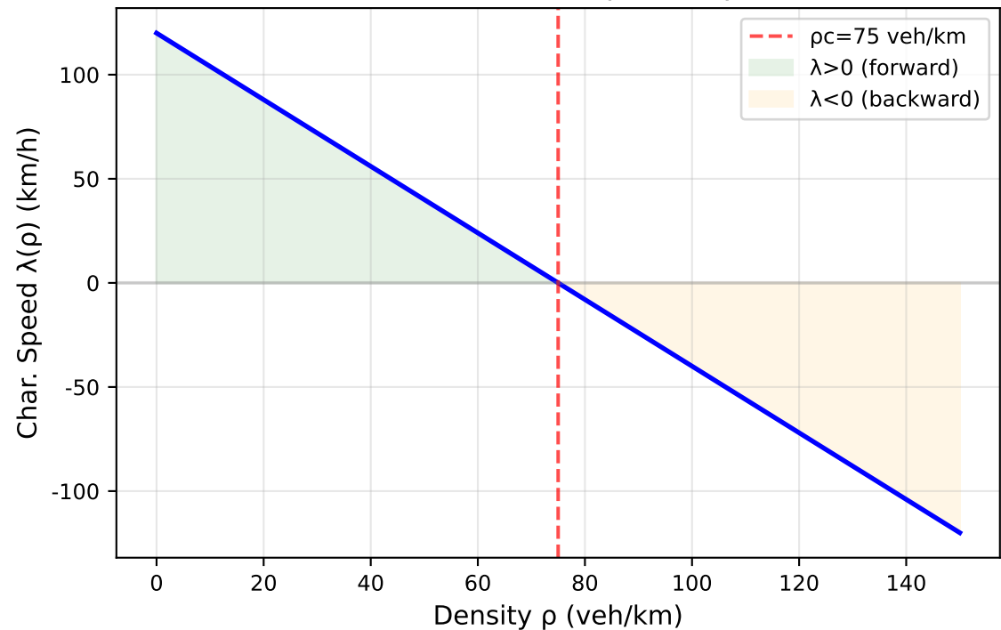
Characteristic Speed \lambda(\rho)
