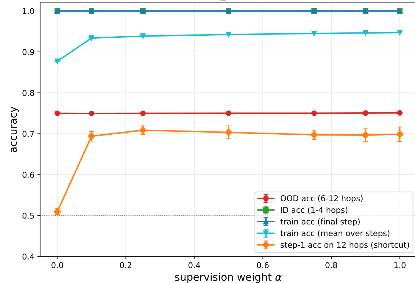
E1: metrics vs \alpha (d_model=128, 3 seeds)
