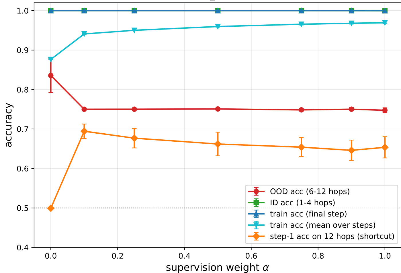
E3: metrics vs \alpha (d_model=256, 5 seeds)
