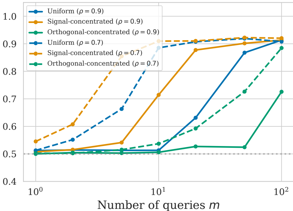
Classification accuracy
