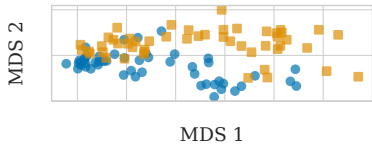
"Orthogonal" queries, m = 10
