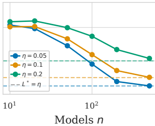
(f) Varying n m=50, r=5, M=100
