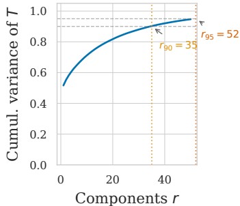
(c) SVD of distance tensor
