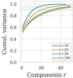
(c) SVD of distance matrix
