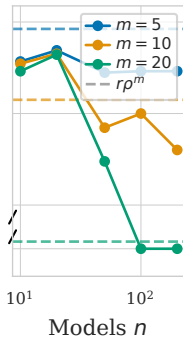
(c) Varying n r=5, \rho=0.7, M=100
