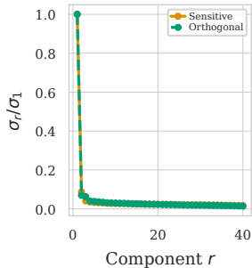
(c) Singular values of D
