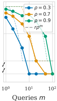
(b) Varying \rho n=100, r=5, M=100
