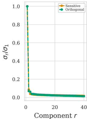
(c) Singular values of D
