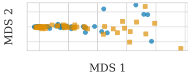
"Orthogonal" queries, m = 5
