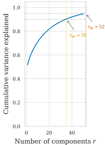
(c) Effective rank
