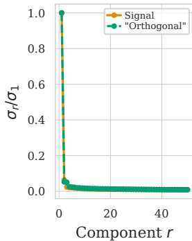
(c) Singular values of D
