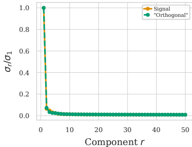
(b) Singular values of D
