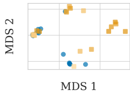
Orthogonal queries
