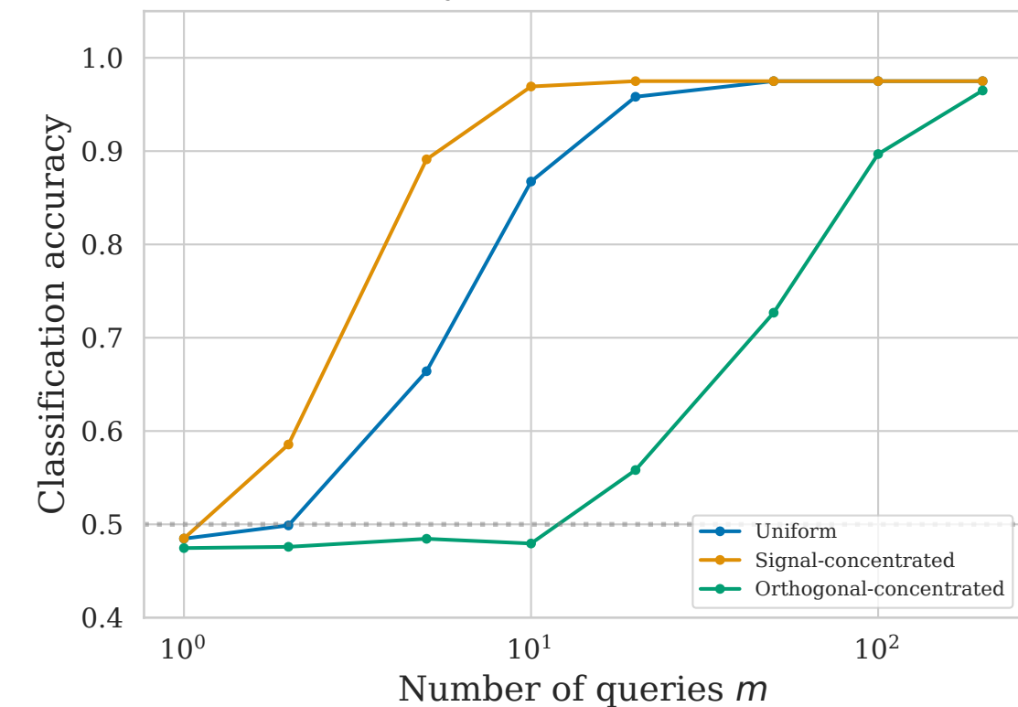
(c) Query distribution ( r = 5, p = 0.3 )
