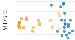
Orthogonal queries
