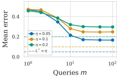
(e) Varying \eta n=100, r=5, M=100
