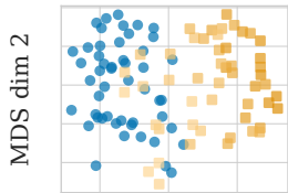
Orthogonal queries
