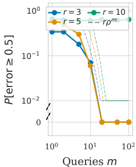
(a) Varying rank r n=100, \rho \approx 0.7, M=100
