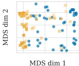
Orthogonal queries
