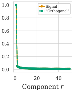
(b) Singular values of D
