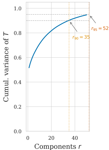
(c) SVD of distance tensor
