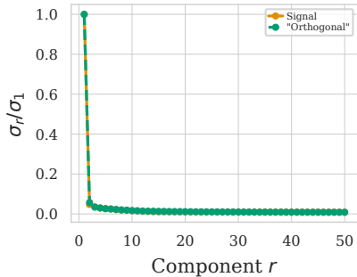
(b) Singular values of D
