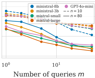
(b) Across base LLMs
