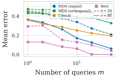
(a) MDS vs. baselines
