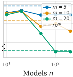
(c) Varying n r=5, \rho=0.7, M=100
