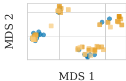
"Orthogonal" queries ( m = 5 )
