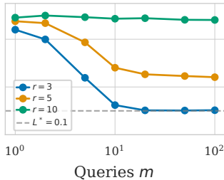
(g) Varying rank r n=100, \eta=0.1, M=100
