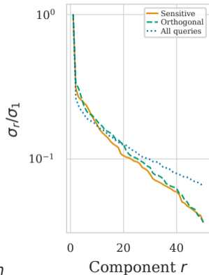
(c) Singular values of D
