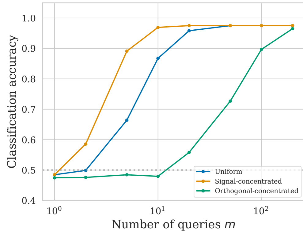
(c) Query distribution ( r = 5, p = 0.3 )
