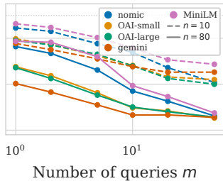
(c) Across embeddings
