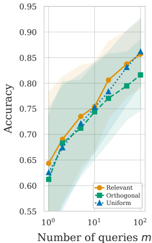
(b) Accuracy vs m
