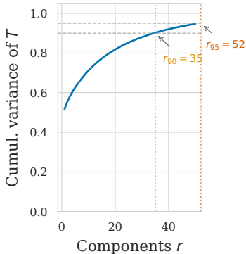
(c) SVD of distance tensor
