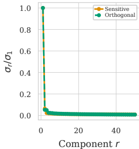
(c) Singular values of D
