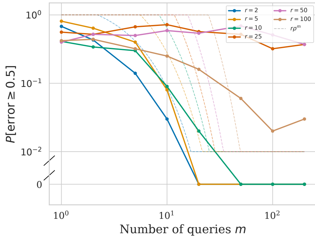
(a) Varying rank r ( p = 0.3 )
