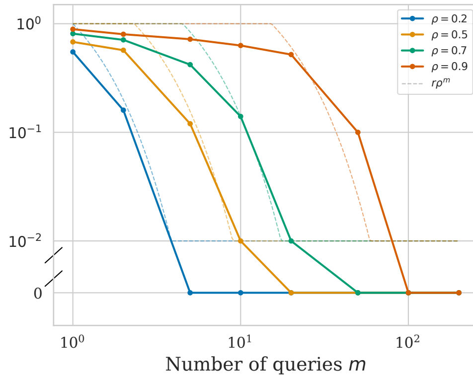
(b) Varying \rho ( r = 5 )
