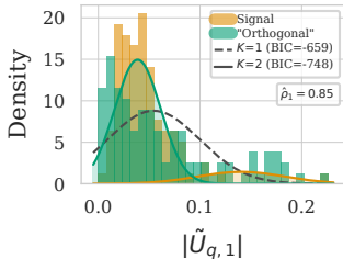
(b) GMM on |\tilde{U}_{q,1}|
