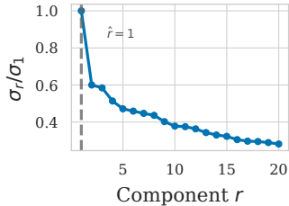
(a) Singular values of \tilde{E}
