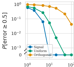
(e) Estimating rank \rho=0.7, n=100
